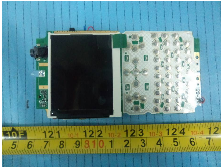
EUT – Main Board with LCD and Keyboard View
