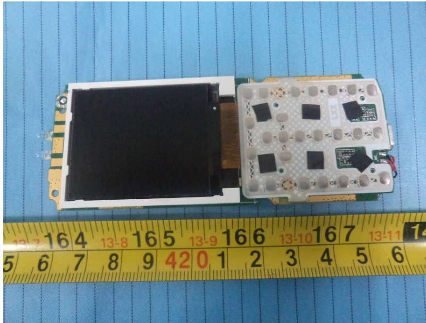
EUT – Main Board Top with Display View
