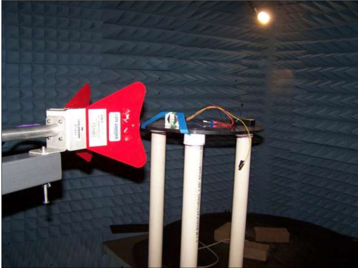
Photograph 2. Radiated Emissions
