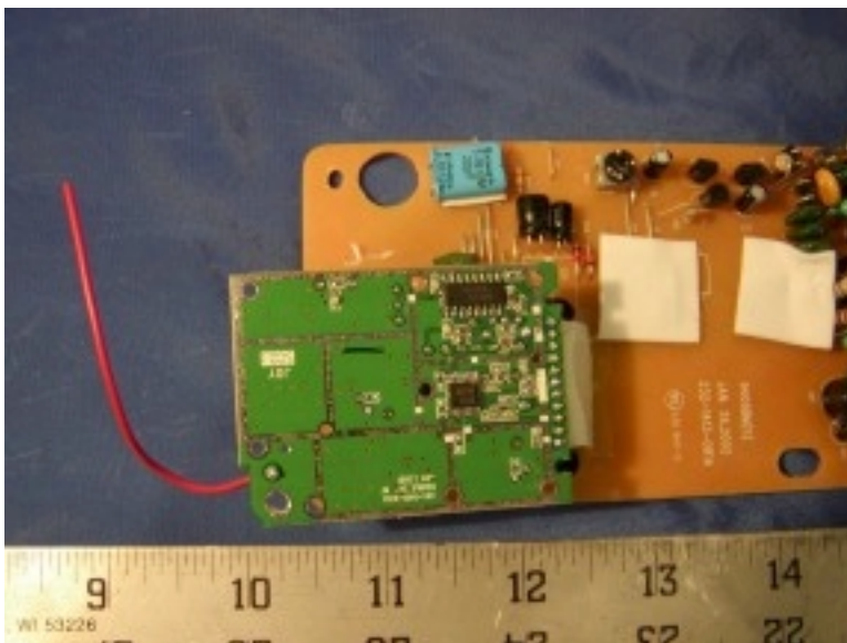
Base - Transceiver Solder View
