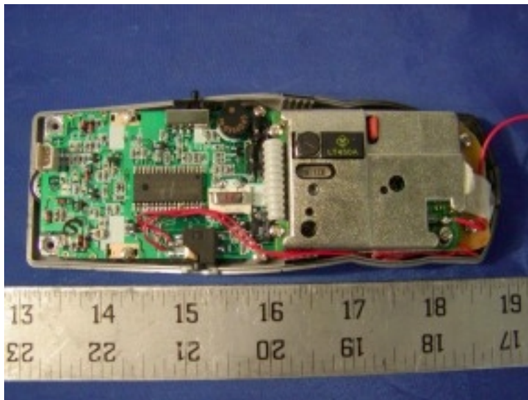
Handset - Component View
