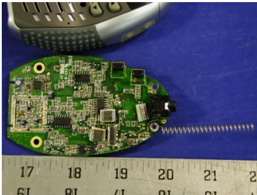
EUT – Solder View with Antenna
