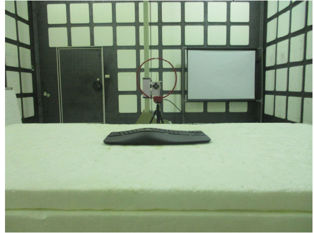
FCC_15_247_BLE_Radiated_Setup
