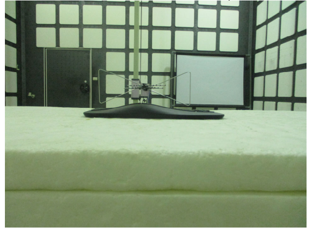
FCC_15.249_2.4G_Radiated_Setup
