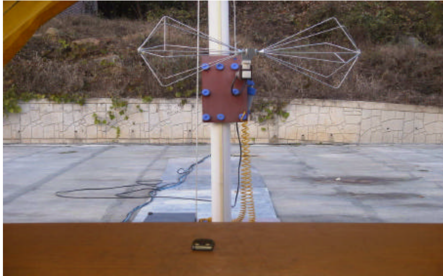
Photograph 1 : Setup for radiated Emissions
