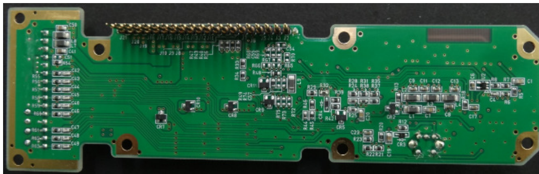
5.10 PCB: E61-500A Top view
