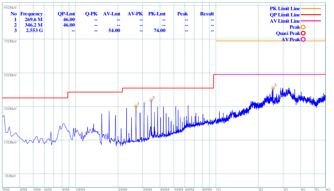
(Plot B: 30MHz – 6GHz, Test Antenna Horizontal)
