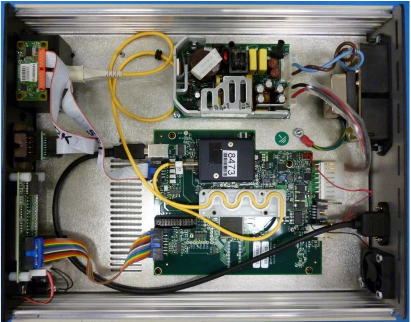
Figure 1: EUT Internal Photo Overview
