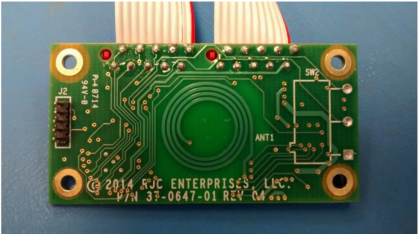
Figure 2: Antenna PCB Front View Note: Antenna is located as indicated "ANT1"
