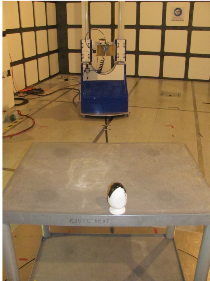
Radiated Emissions 1-3GHz
