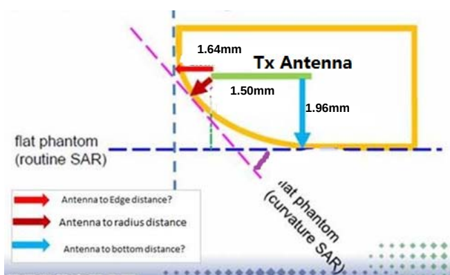
X=1.64mm, Y=1.96mm, Z=1.50mm Exterior Radius Dimension for WWAN
