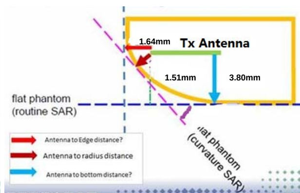
X=1.64mm, Y=3.80mm, Z=1.51mm Exterior Radius Dimension for WLAN2
