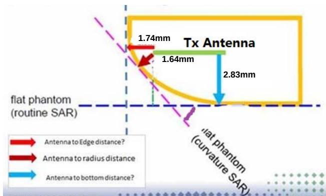
X=1.74mm, Y=2.83mm, Z=1.64mm Exterior Radius Dimension for WLAN1
