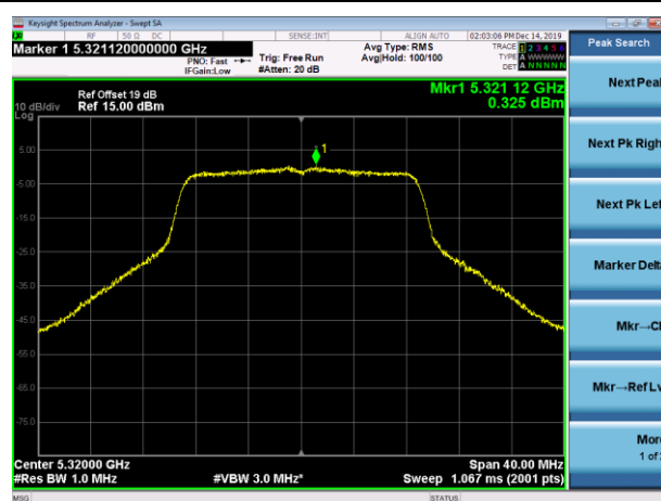
Channel 64 (5320MHz)
