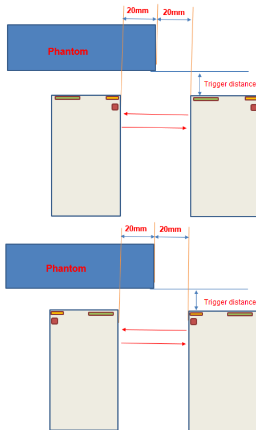
proximity sensor coverage assesment (X coordinate direction)
