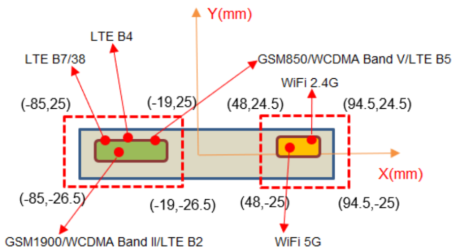
sensor coverage assesment results(Top side):
