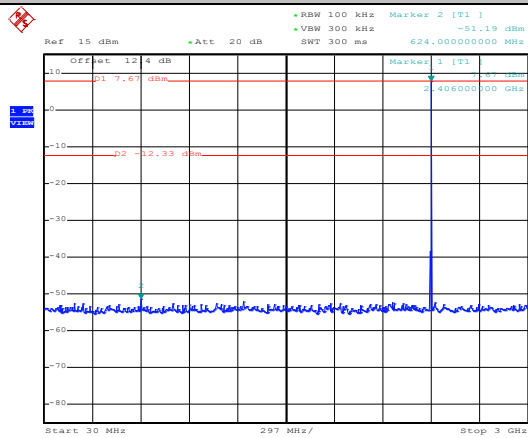
CSE Plot on CH 00 between 30 MHz ~ 3 GHz
