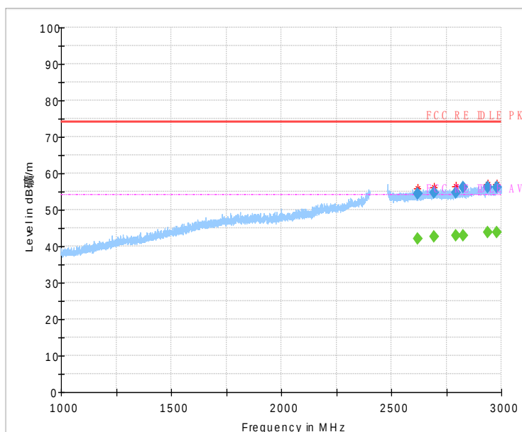
Fig.22 Radiated emission: Ch39, 1GHz~3GHz
