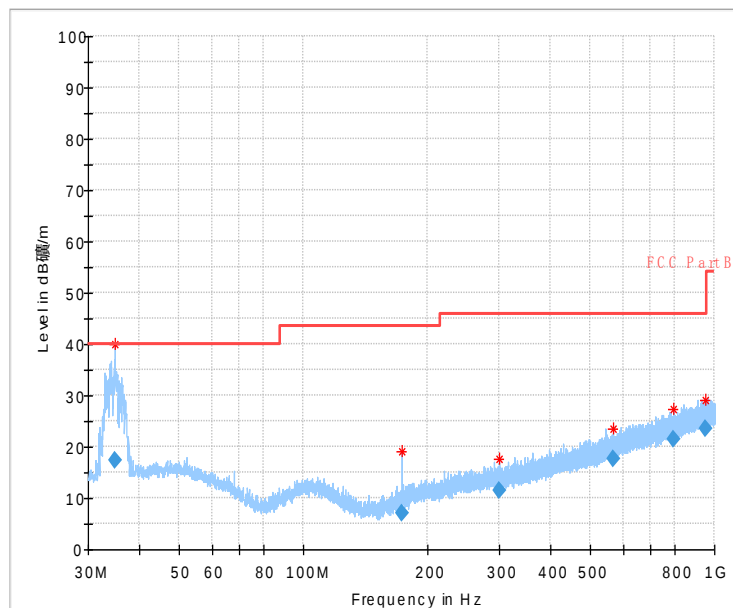
Fig.21 Radiated emission: Ch39, 30MHz~1GHz
