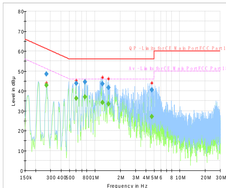
Fig.24 AC Powerline Conducted Emission
