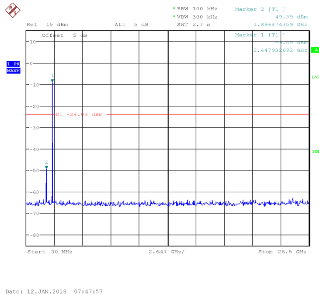
Fig.17 Conducted spurious emission: Ch39, 30MHz~26GHz
