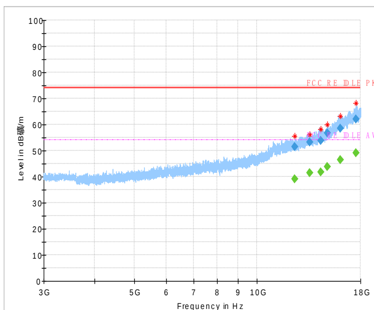
Fig.23 Radiated emission: Ch39, 3GHz~18GHz
