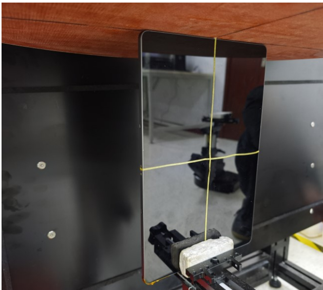
Edge4, Test Separation 0 mm
