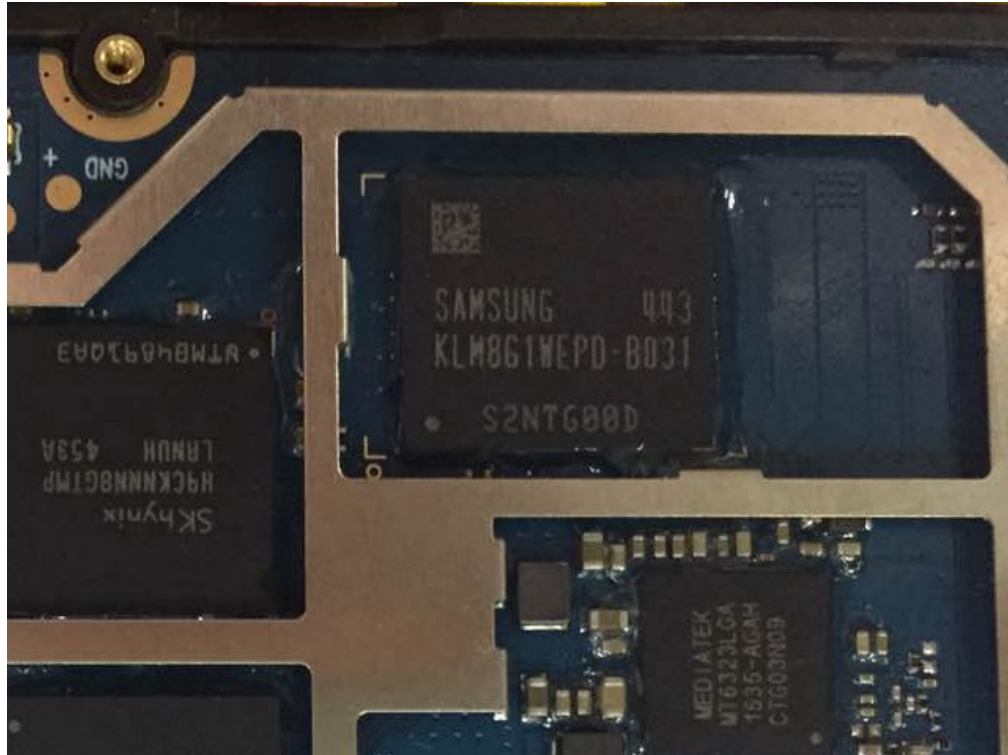
Memory-EMMC(8GB)
