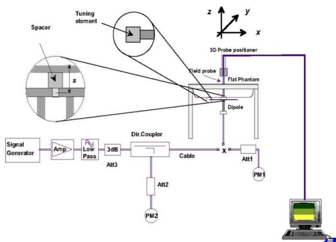
Fig 8.3.1 System Performance Check Setup
