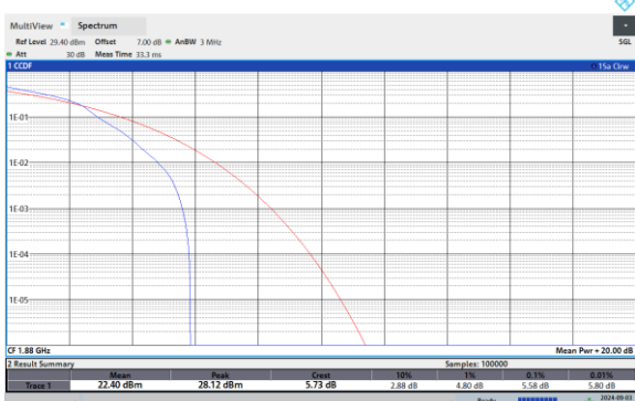
Band25-3MHz-16QAM-26675-1RB#0
