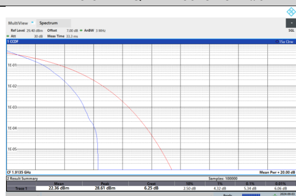
Band25-3MHz-16QAM-26055-15RB#0
