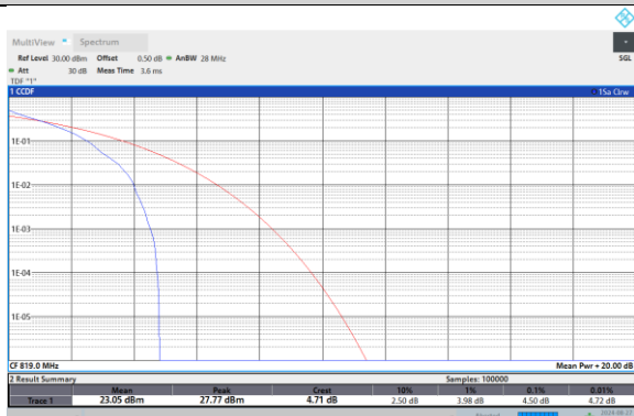
Band26-10MHz-16QAM-26740-1RB#0
