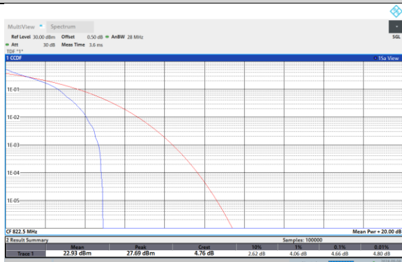
Band26-3MHz-16QAM-26705-1RB#0
