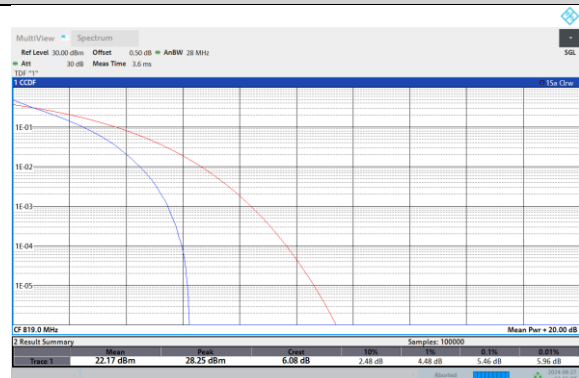
Band26-10MHz-16QAM-26740-50RB#0
