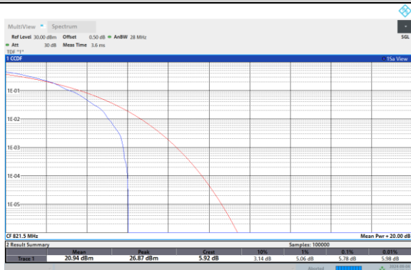
Band26-10MHz-QPSK-26740-1RB#0
