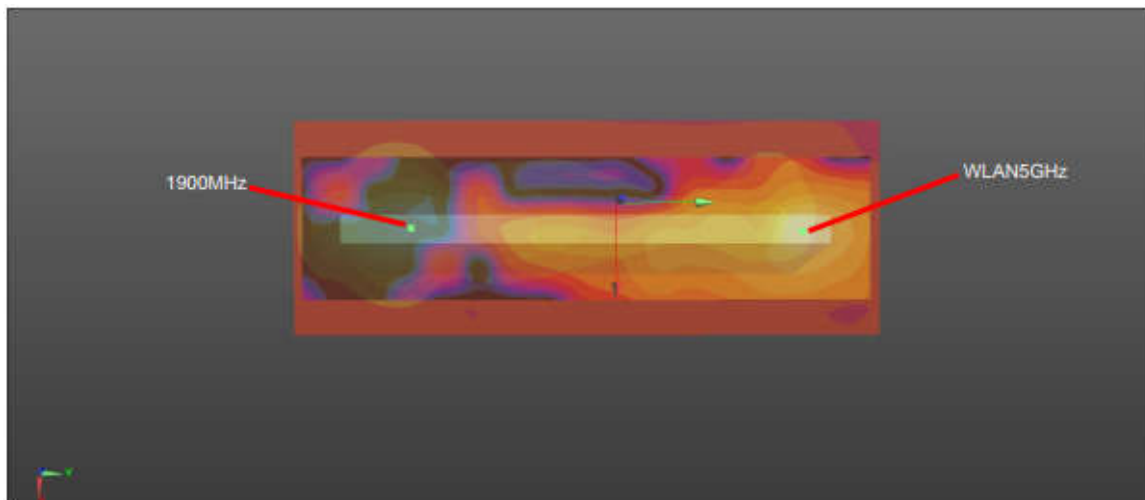
WWAN+WLAN5GHz_Edge 1
