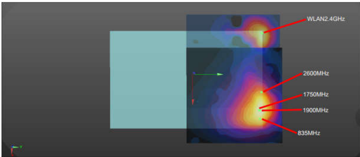
WWAN+ WLAN2.4GHz _Bottom Face
