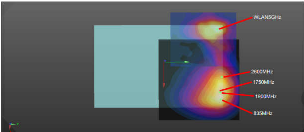
WWAN+ WLAN5GHz _Bottom Face
