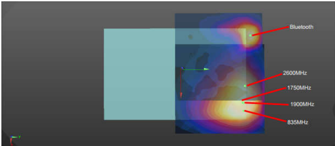
WWAN+BT_Bottom Face
