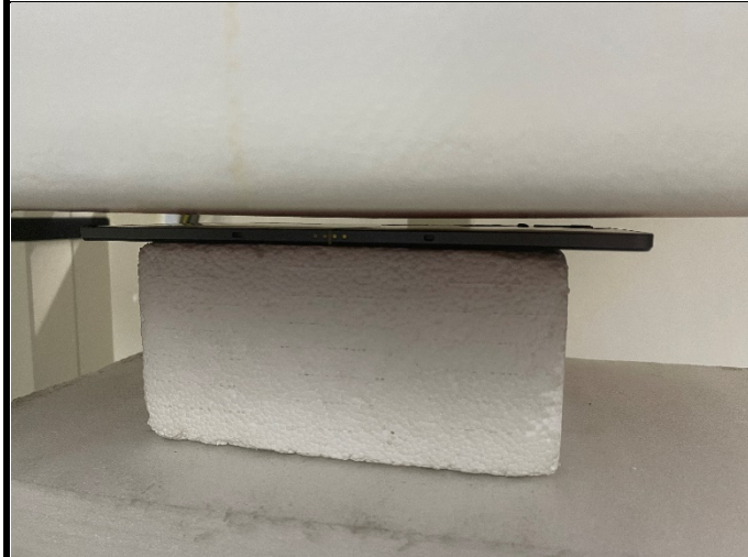
Rear Face of EUT with 0.7 cm Gap
