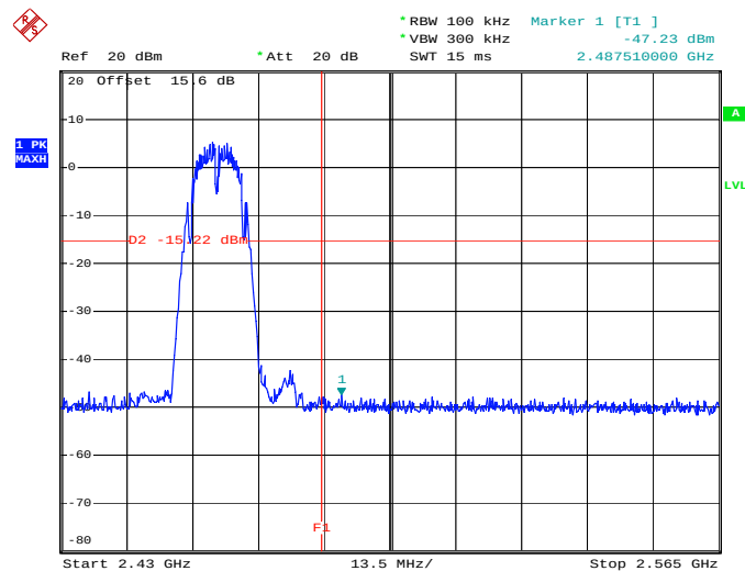
High Band Edge Plot on 802.11b Channel 11
