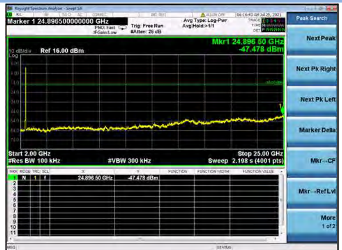
802.11g CHANNEL 12, SPURIOUS 2 GHz ~ 25 GHz
