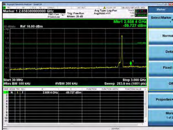
802.11g CHANNEL 12, SPURIOUS 30 MHz ~ 3 GHz
