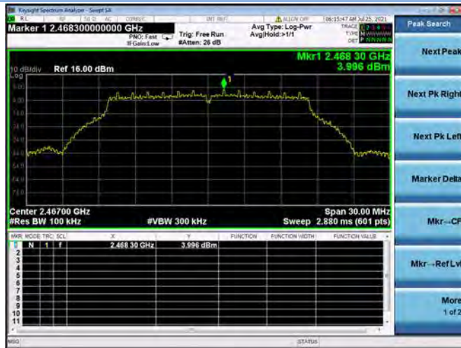
802.11g CHANNEL 12 CARRIER LEVEL
