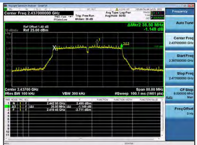
802.11n-40 MHz CHANNEL 6
