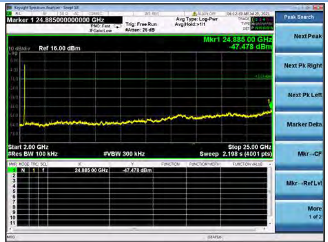
802.11g CHANNEL 11, SPURIOUS 2 GHz ~ 25 GHz
