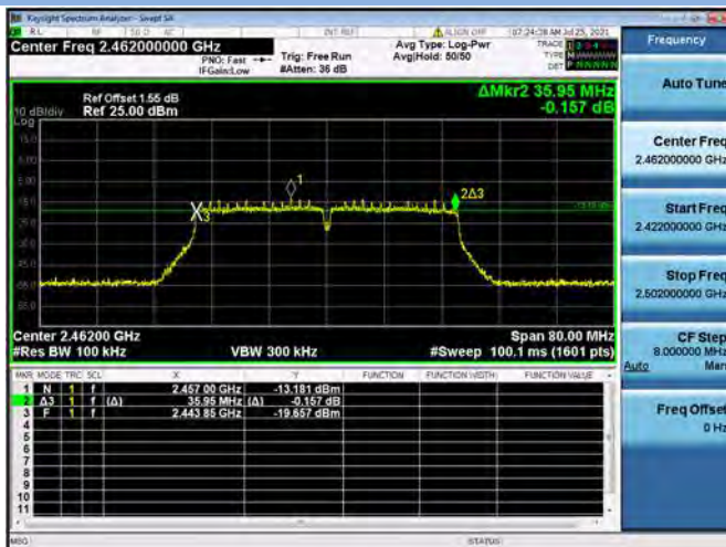
802.11n-40 MHz CHANNEL 11
