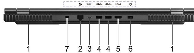
Figure 8. Lenovo Legion 5 (17", 05) - rear view
