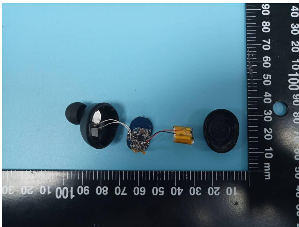
Right Earbud
