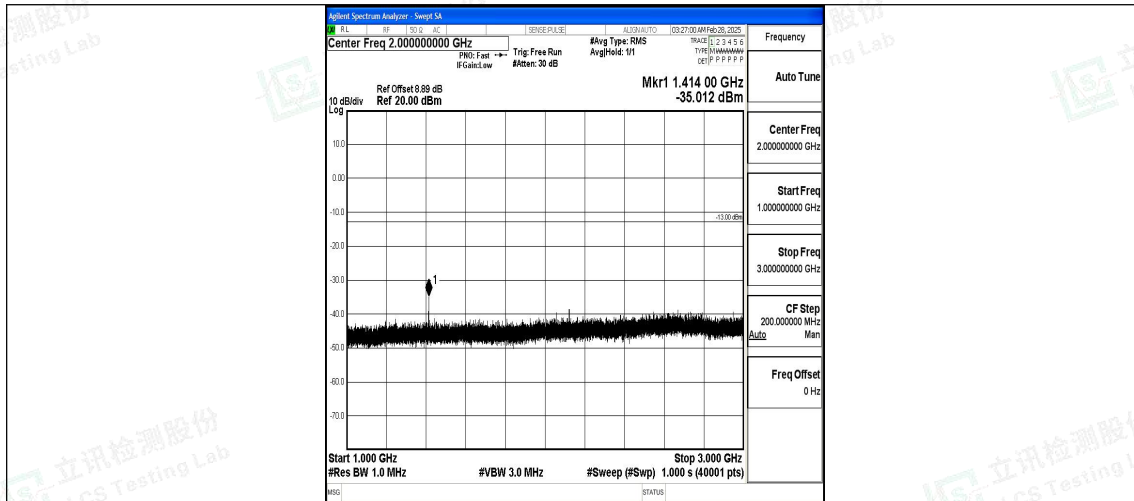
Band12_1.4MHz_16QAM_23095_1RB#0_1000~3000_1000~3000
