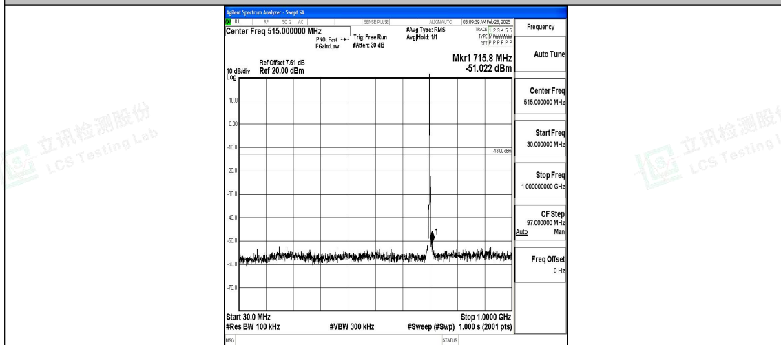
Band12_3MHz_16QAM_23095_1RB#0_30~1000_30~1000
