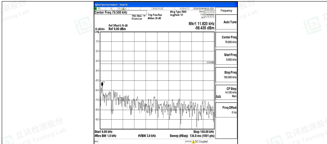
Band12_3MHz_16QAM_23095_1RB#0_0.009~0.15_0.009~0.15
