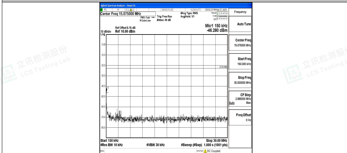
Band5_10MHz_16QAM_20525_1RB#0_0.15~30_0.15~30
