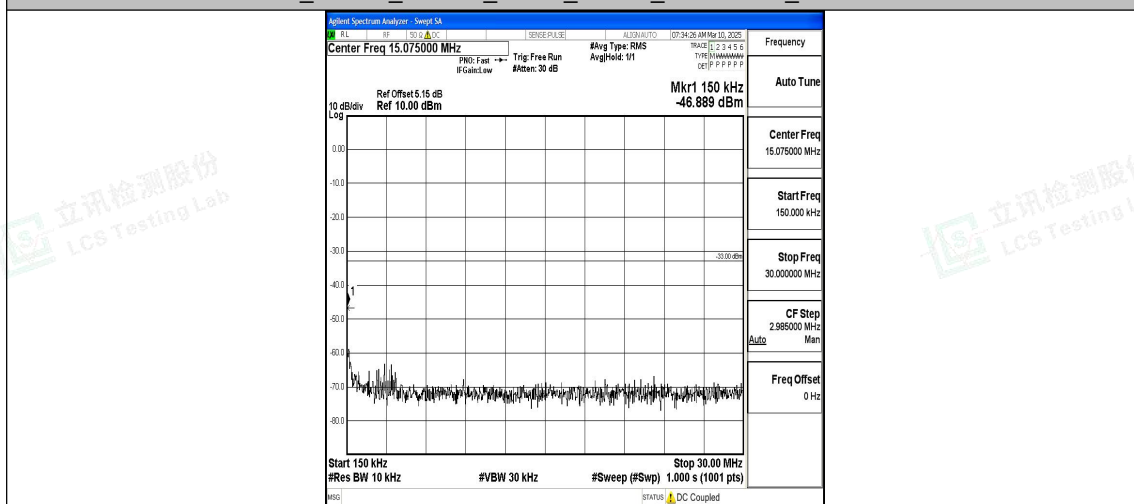
Band4_15MHz_16QAM_20025_1RB#0_0.15~30_0.15~30
