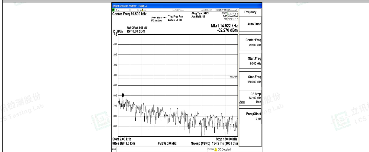
Band66_20MHz_QPSK_132572_1RB#0_0.009~0.15_0.009~0.15
