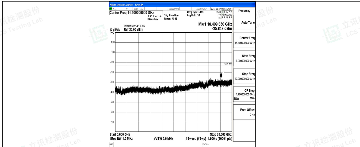
Band66_20MHz_16QAM_132322_1RB#0_3000~20000_3000~20000
