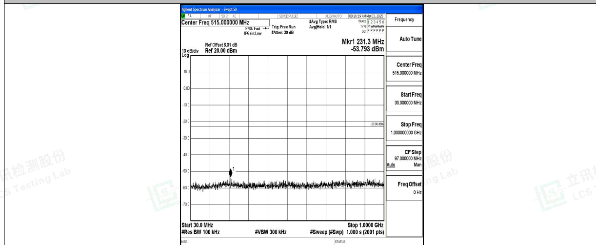
Band66_10MHz_QPSK_132022_1RB#0_30~1000_30~1000
