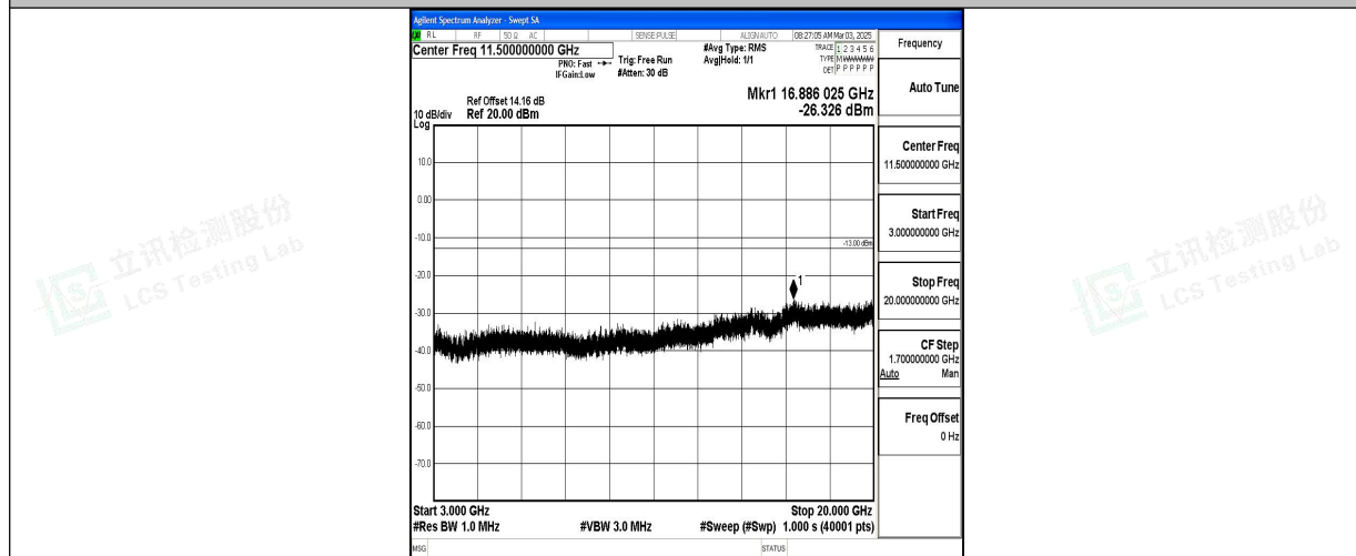
Band66_10MHz_16QAM_132022_1RB#0_3000~20000_3000~20000
