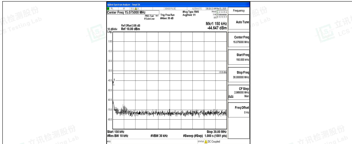
Band66_10MHz_QPSK_132022_1RB#0_0.15~30_0.15~30
