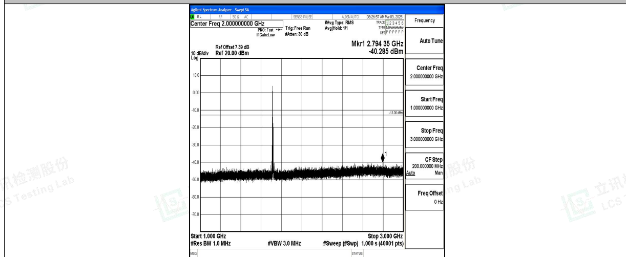
Band66_10MHz_16QAM_132022_1RB#0_1000~3000_1000~3000
