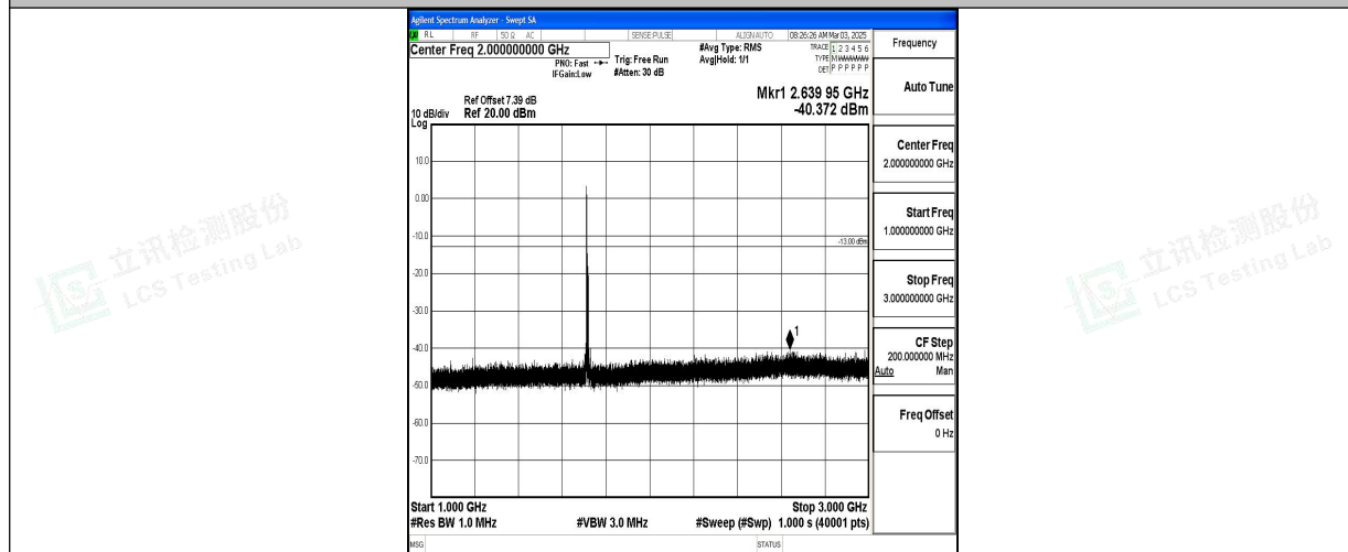
Band66_10MHz_QPSK_132022_1RB#0_1000~3000_1000~3000
