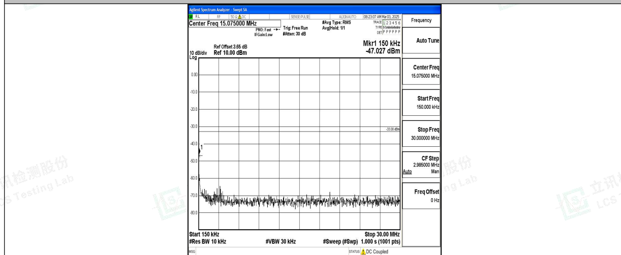
Band66_5MHz_QPSK_132322_1RB#0_0.15~30_0.15~30
