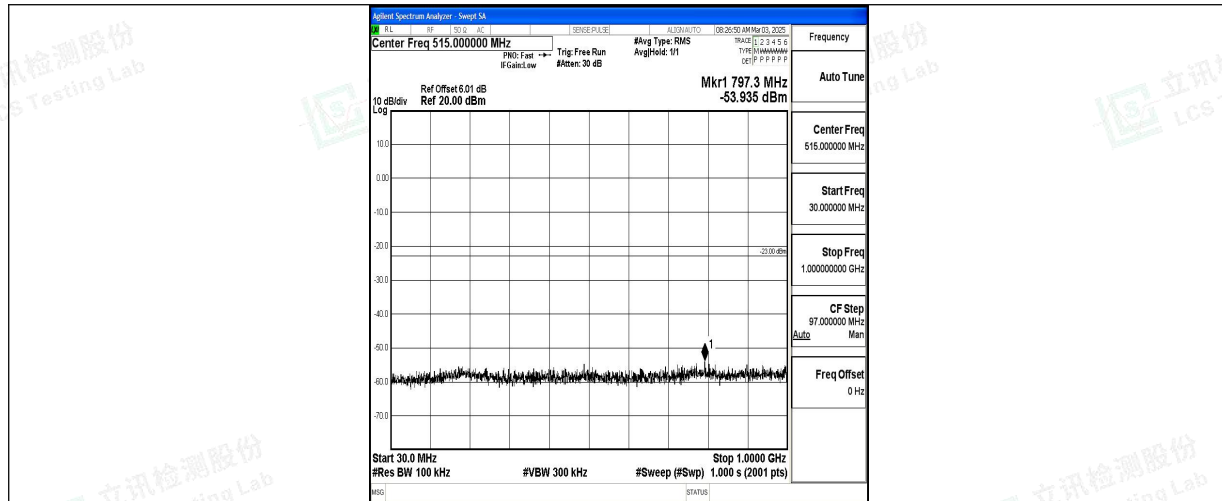
Band66_10MHz_16QAM_132022_1RB#0_30~1000_30~1000
