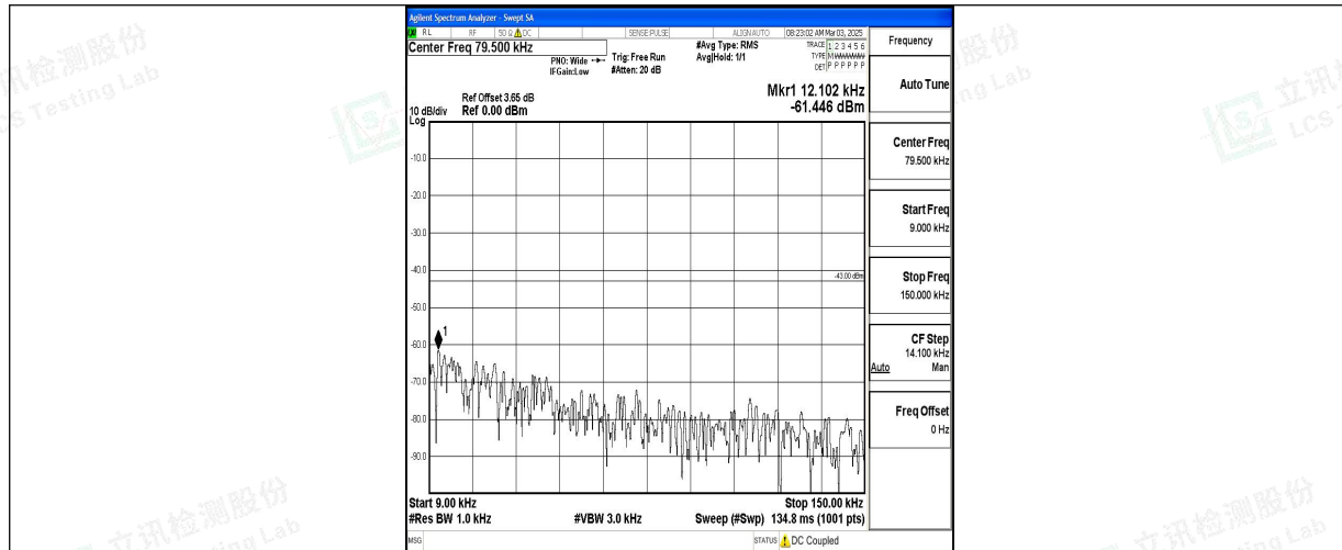
Band66_5MHz_QPSK_132322_1RB#0_0.009~0.15_0.009~0.15
