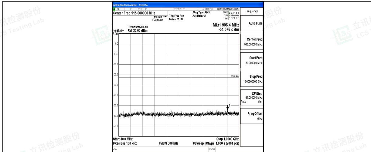
Band66_1.4MHz_QPSK_132665_1RB#0_30~1000_30~1000
