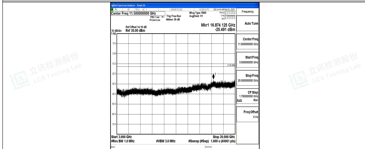
Band66_1.4MHz_QPSK_132665_1RB#0_3000~20000_3000~20000
