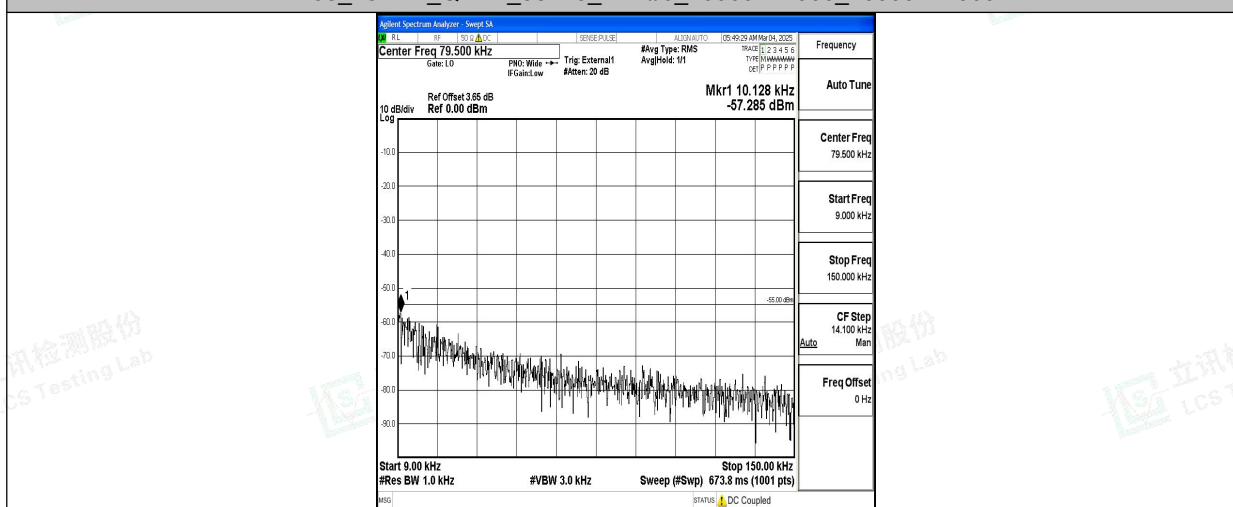
Band38_15MHz_16QAM_38175_1RB#0_0.009~0.15_0.009~0.15
