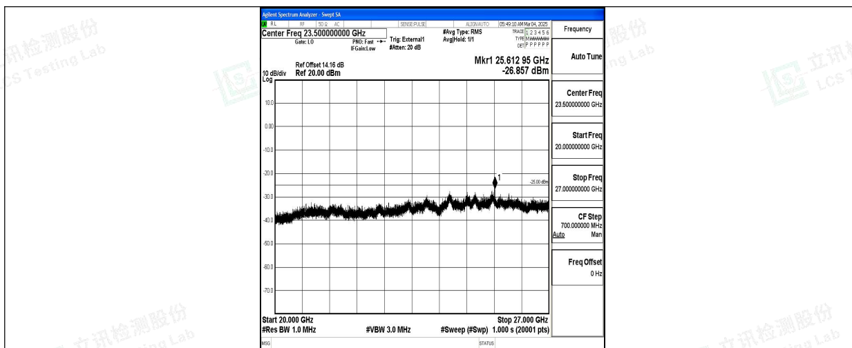
Band38_15MHz_QPSK_38175_1RB#0_20000~27000_20000~27000
