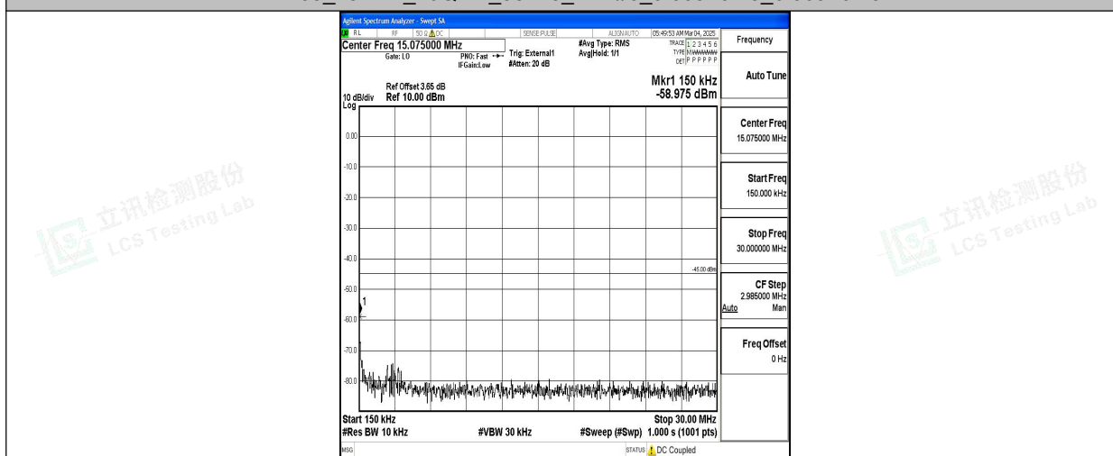
Band38_15MHz_16QAM_38175_1RB#0_0.15~30_0.15~30
