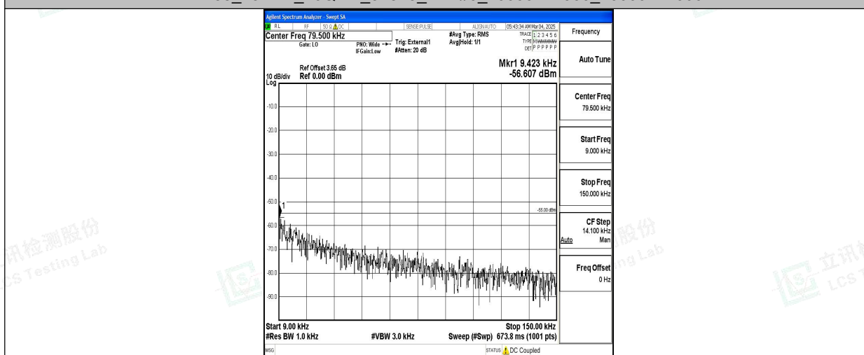
Band38_15MHz_QPSK_38000_1RB#0_0.009~0.15_0.009~0.15
