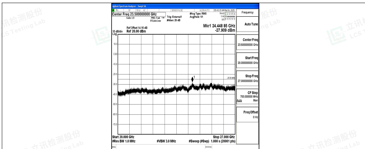
Band38_15MHz_16QAM_37825_1RB#0_20000~27000_20000~27000
