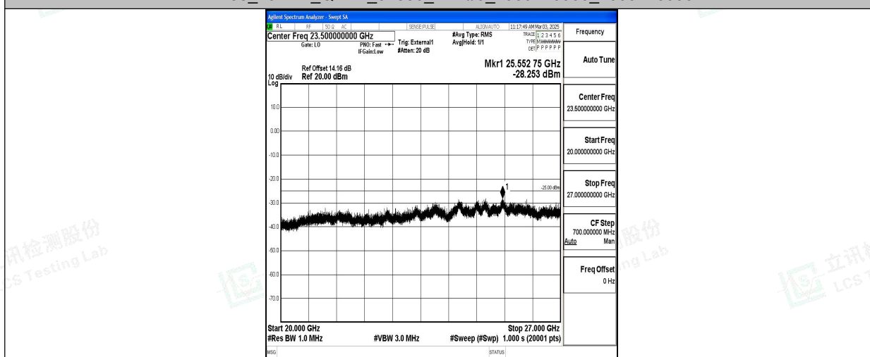
Band38_20MHz_QPSK_37850_1RB#0_20000~27000_20000~27000
