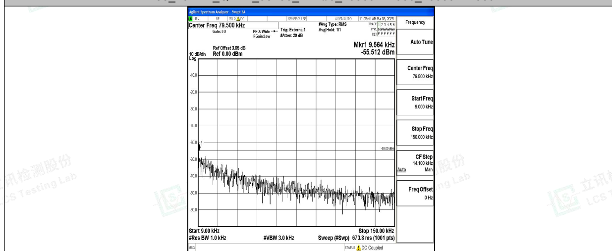
Band38_20MHz_16QAM_38150_1RB#0_0.009~0.15_0.009~0.15
