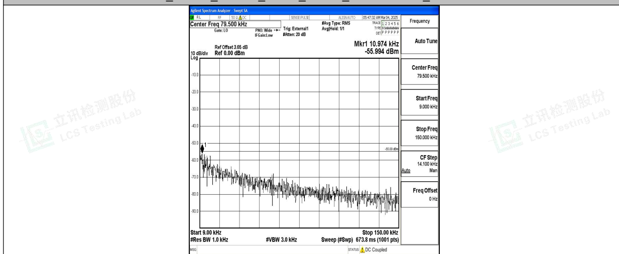
Band38_15MHz_QPSK_38175_1RB#0_0.009~0.15_0.009~0.15
