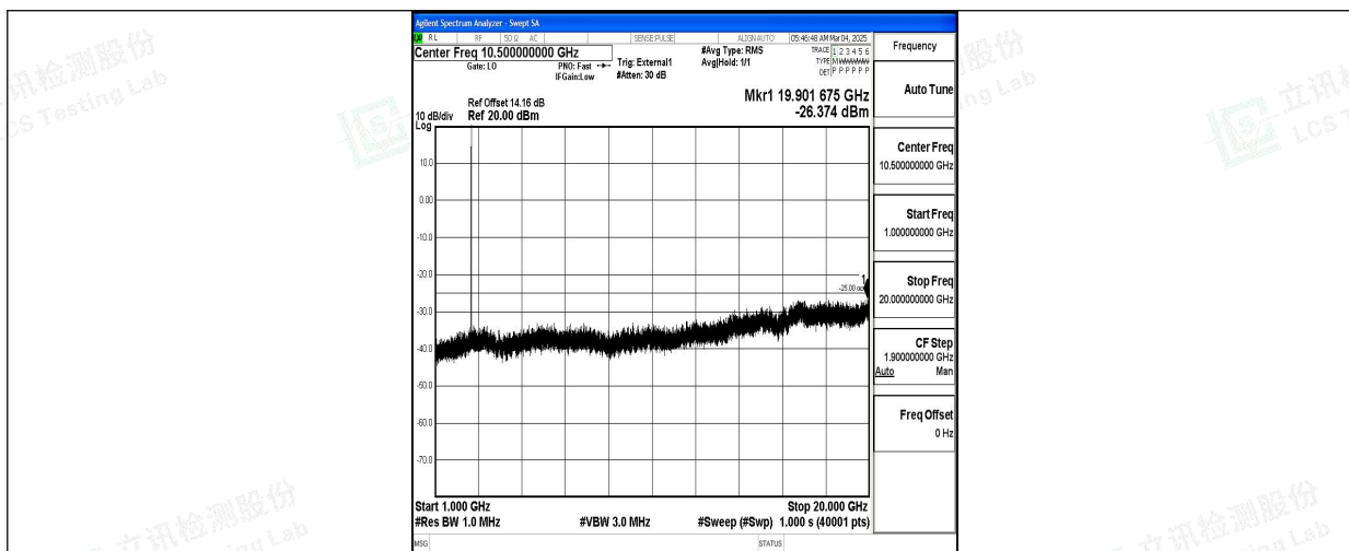
Band38_15MHz_16QAM_38000_1RB#0_1000~20000_1000~20000
