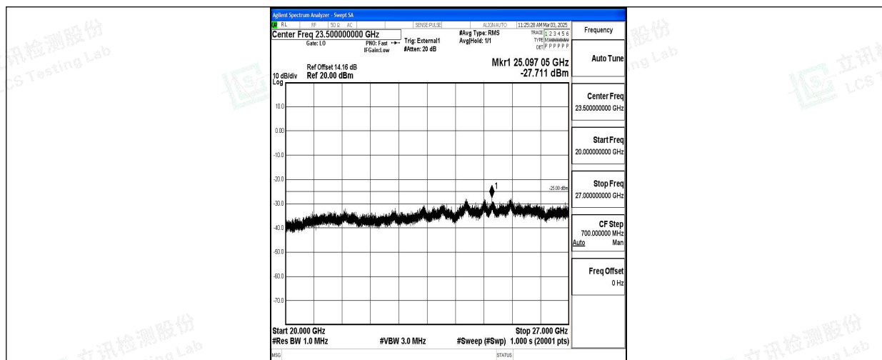
Band38_20MHz_QPSK_38150_1RB#0_20000~27000_20000~27000
