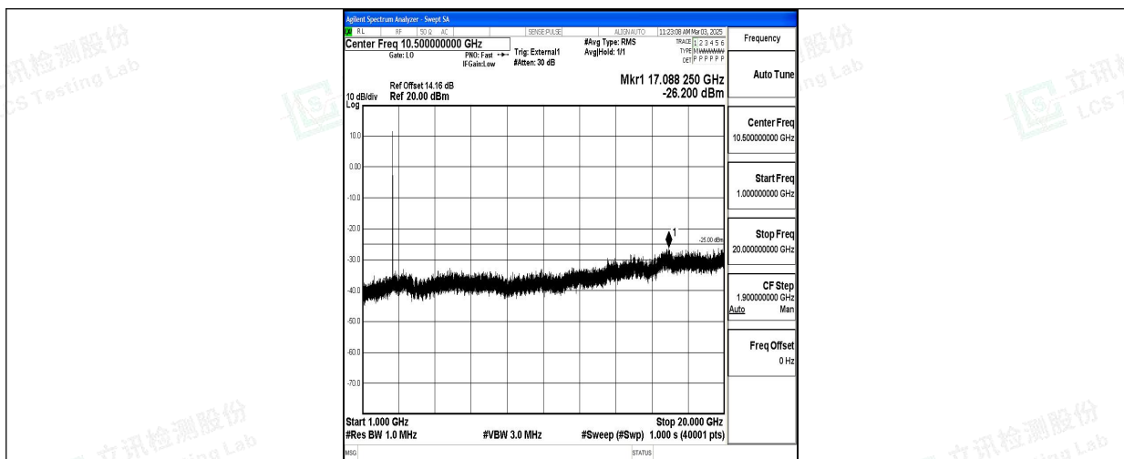
Band38_20MHz_16QAM_38000_1RB#0_1000~20000_1000~20000
