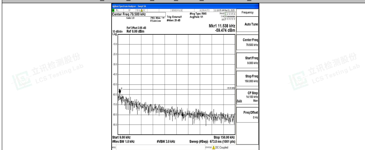
Band38_20MHz_16QAM_37850_1RB#0_0.009~0.15_0.009~0.15
