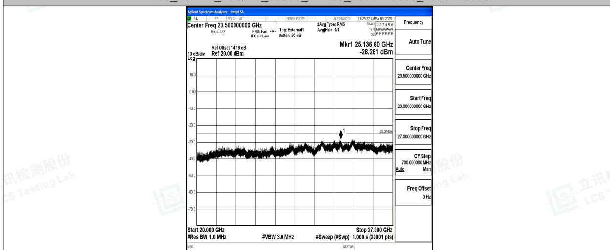
Band38_20MHz_16QAM_38000_1RB#0_20000~27000_20000~27000
