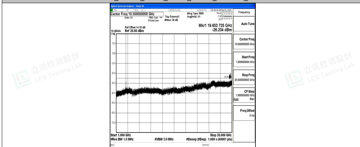
Band38_15MHz_QPSK_38175_1RB#0_1000~20000_1000~20000
