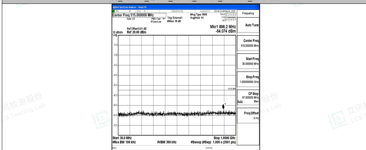
Band38_15MHz_QPSK_38175_1RB#0_30~1000_30~1000
