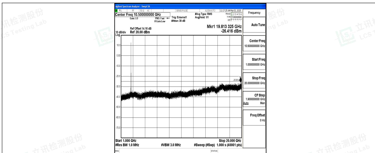
Band38_20MHz_QPSK_37850_1RB#0_1000~20000_1000~20000
