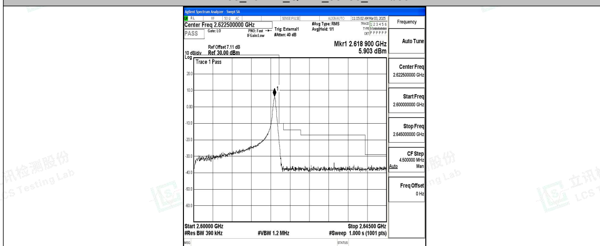
Band38_20MHz_16QAM_38150_1RB#99
