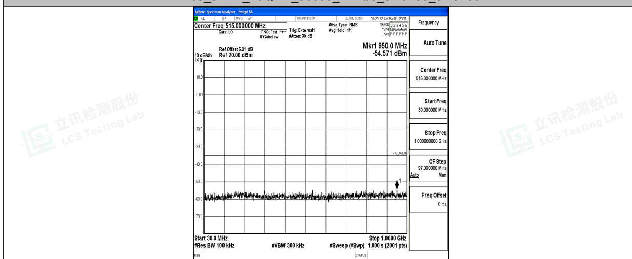
Band38_5MHz_16QAM_38000_1RB#0_30~1000_30~1000
