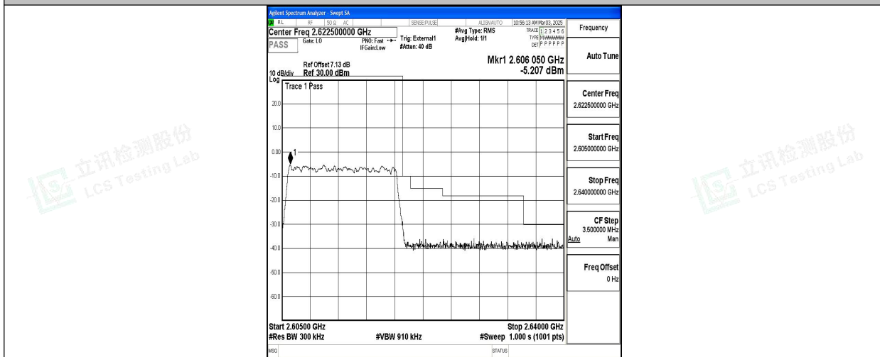
Band38_15MHz_QPSK_38175_75RB#0
