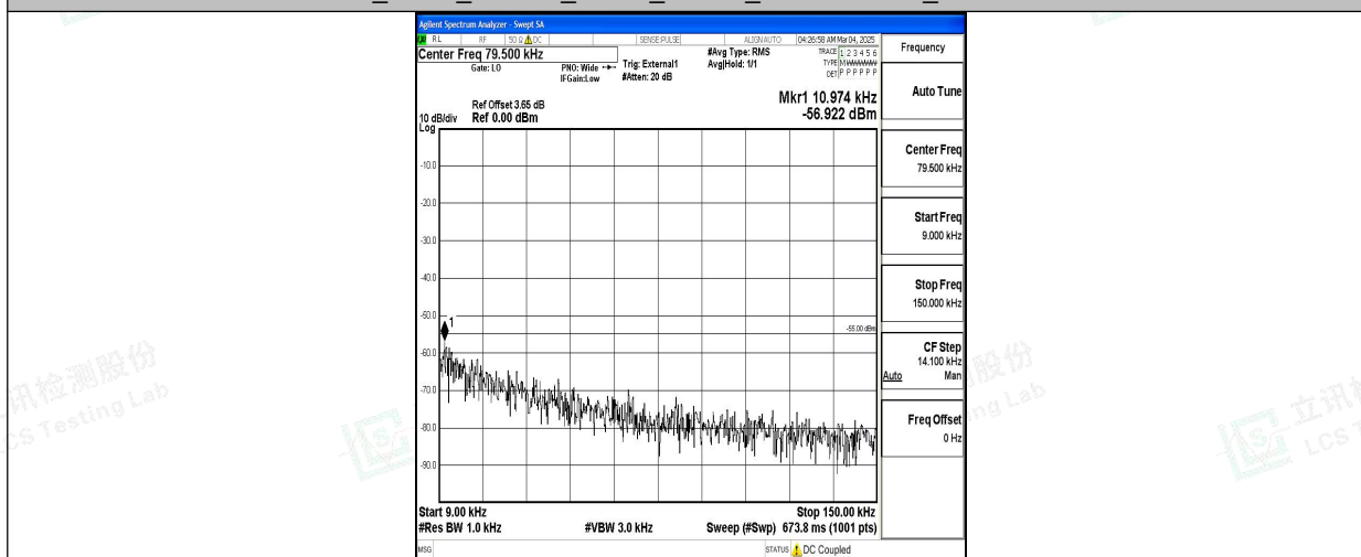
Band38_5MHz_QPSK_38000_1RB#0_0.009~0.15_0.009~0.15
