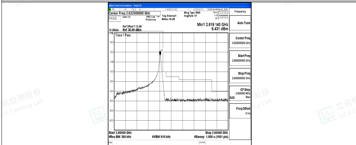
Band38_15MHz_16QAM_38175_1RB#74
