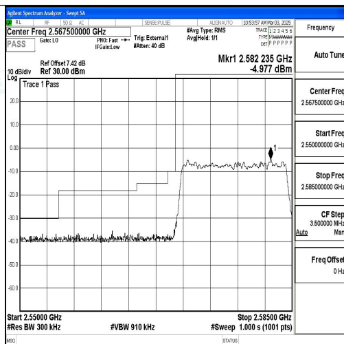
Band38_15MHz_16QAM_37825_75RB#0
