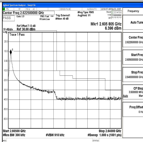
Band38_15MHz_16QAM_38175_1RB#0
