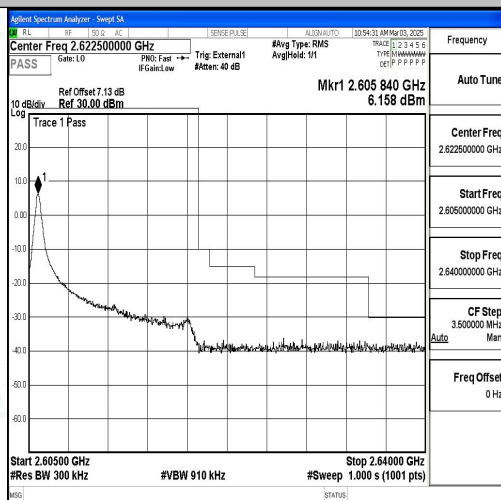
Band38_15MHz_QPSK_38175_1RB#0
