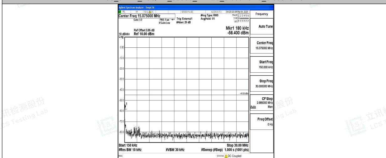
Band38_5MHz_16QAM_38000_1RB#0_0.15~30_0.15~30
