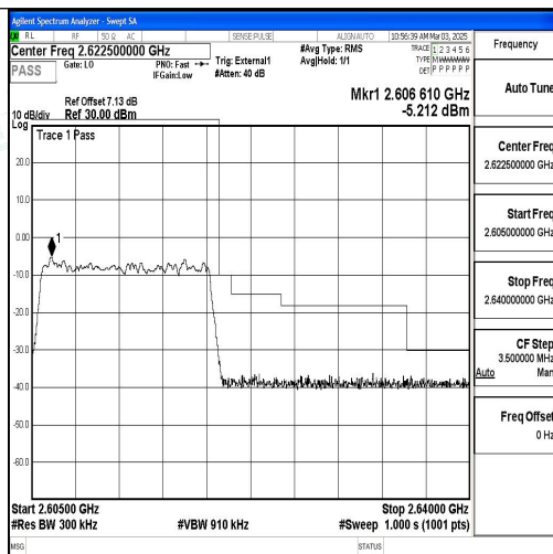
Band38 15MHz 16QAM 38175 75RB#0
