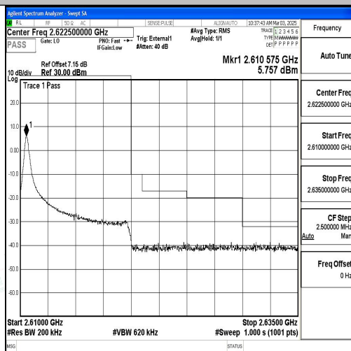
Band38_10MHz_QPSK_38200_1RB#0
