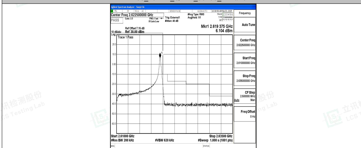
Band38_10MHz_16QAM_38200_1RB#49
