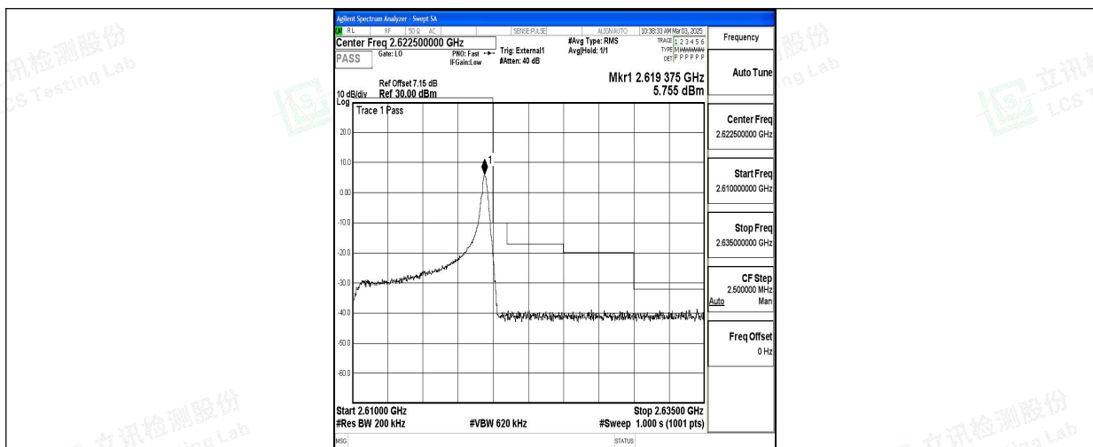
Band38_10MHz_QPSK_38200_1RB#49
