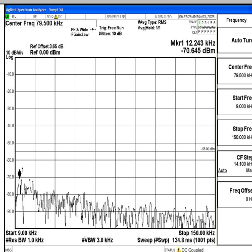
Band7_20MHz_QPSK_21350_1RB#0_0.009~0.15_0.009~0.15
