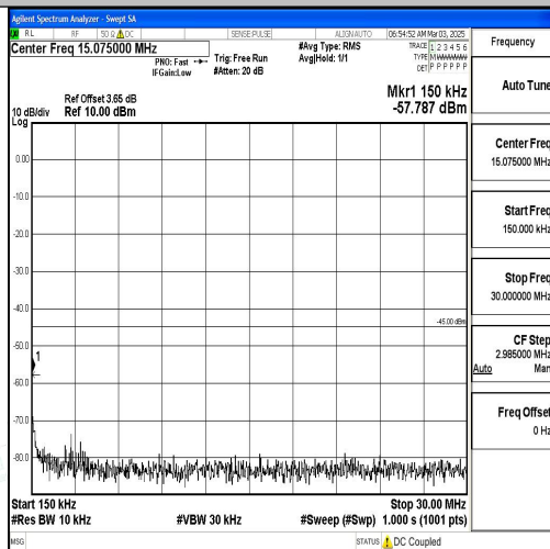
Band7_20MHz_16QAM_21100_1RB#0_0.15~30_0.15~30
