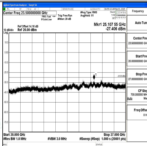
Band7_20MHz_16QAM_21100_1RB#0_20000~27000_20000~27000
