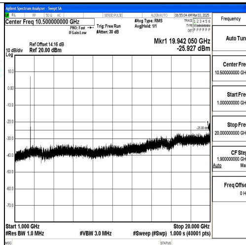
Band7_20MHz_16QAM_21100_1RB#0_1000~20000_1000~20000
