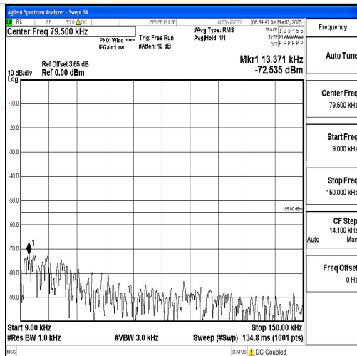
Band7_20MHz_16QAM_21100_1RB#0_0.009~0.15_0.009~0.15
