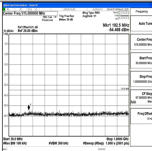
Band7_20MHz_16QAM_21100_1RB#0_30~1000_30~1000
