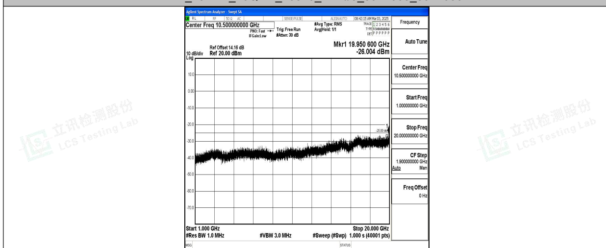
Band7_15MHz_16QAM_20825_1RB#0_1000~20000_1000~20000
