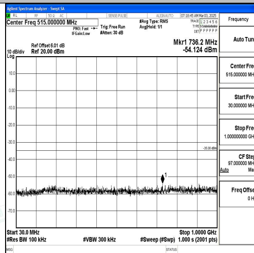
Band7_15MHz_QPSK_21375_1RB#0_30~1000_30~1000
