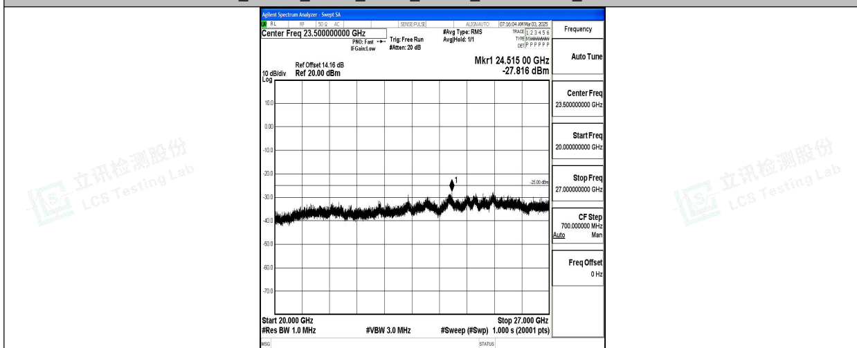
Band7_15MHz_QPSK_21100_1RB#0_20000~27000_20000~27000
