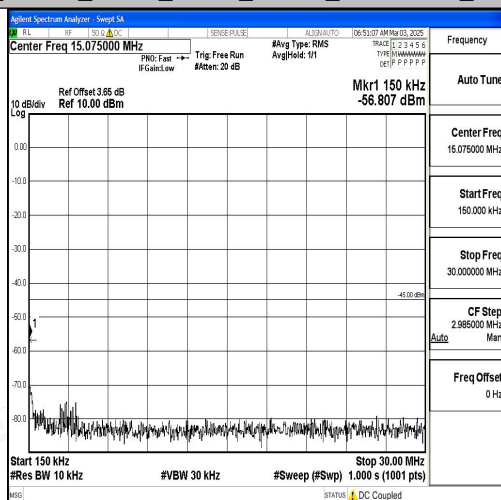
Band7_20MHz_QPSK_20850_1RB#0_0.15~30_0.15~30
