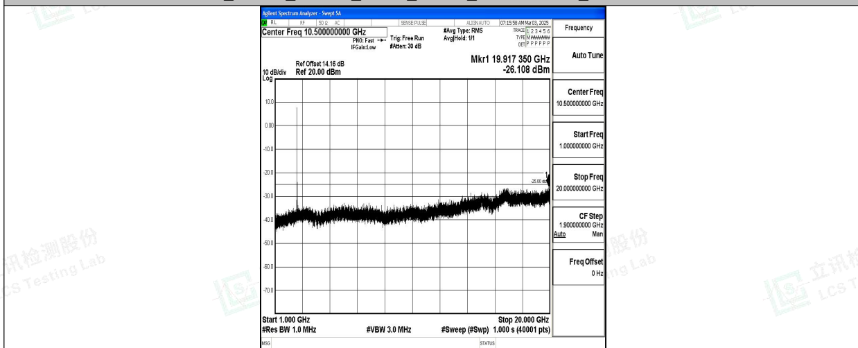
Band7_15MHz_QPSK_21100_1RB#0_1000~20000_1000~20000
