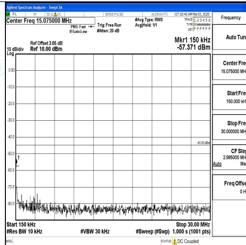
Band7_15MHz_QPSK_21375_1RB#0_0.15~30_0.15~30
