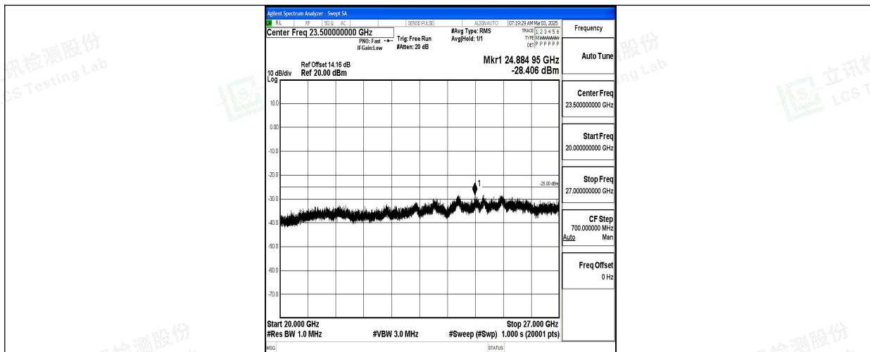
Band7_15MHz_16QAM_21375_1RB#0_20000~27000_20000~27000
