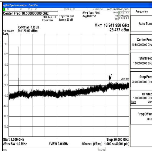
Band7_20MHz_QPSK_20850_1RB#0_1000~20000_1000~20000
