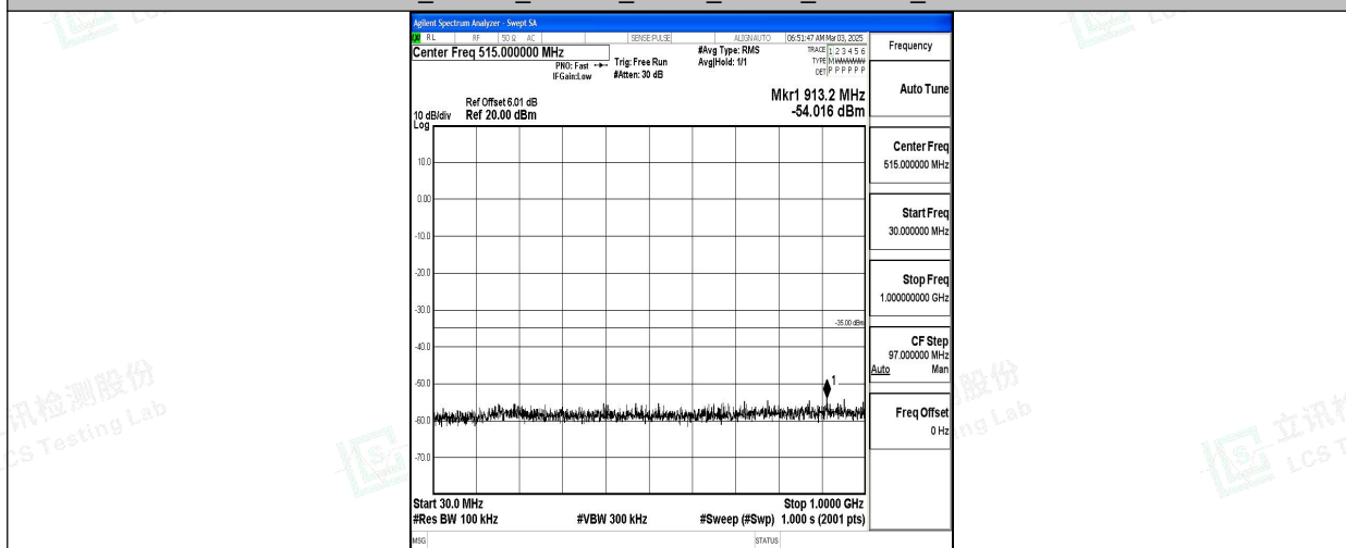
Band7_20MHz_16QAM_20850_1RB#0_30~1000_30~1000
