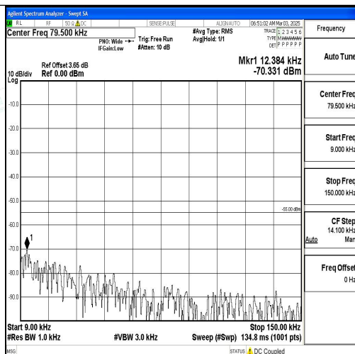
Band7_20MHz_QPSK_20850_1RB#0_0.009~0.15_0.009~0.15
