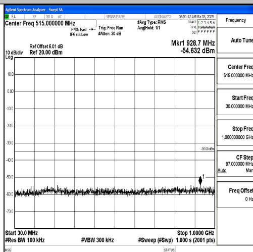
Band7_20MHz_QPSK_20850_1RB#0_30~1000_30~1000
