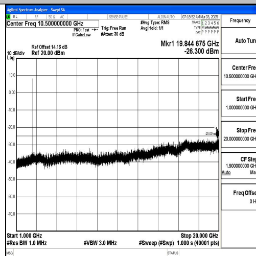
Band7_15MHz_QPSK_21375_1RB#0_1000~20000_1000~20000
