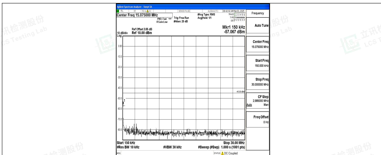
Band7_15MHz_16QAM_20825_1RB#0_0.15~30_0.15~30
