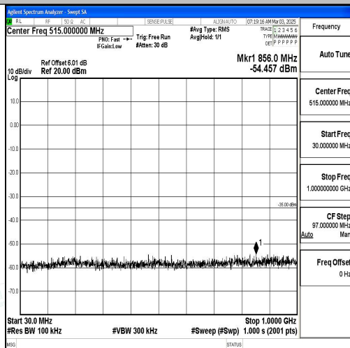
Band7_15MHz_16QAM_21375_1RB#0_30~1000_30~1000
