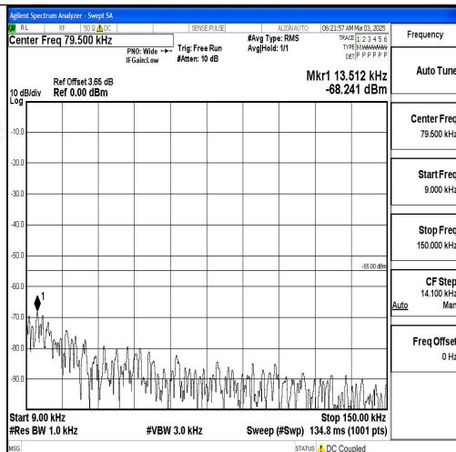
Band7_10MHz_QPSK_20800_1RB#0_0.009~0.15_0.009~0.15
