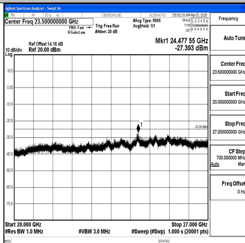
Band7_5MHz_QPSK_21100_1RB#0_20000~27000_20000~27000
