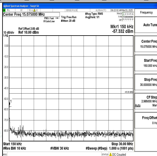
Band7_10MHz_QPSK_20800_1RB#0_0.15~30_0.15~30
