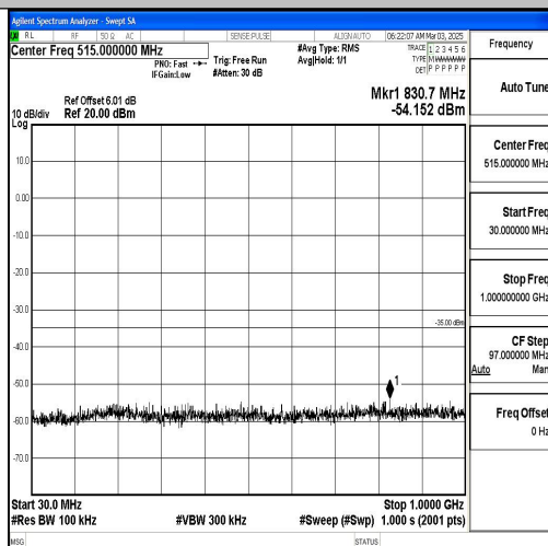
Band7_10MHz_QPSK_20800_1RB#0_30~1000_30~1000
