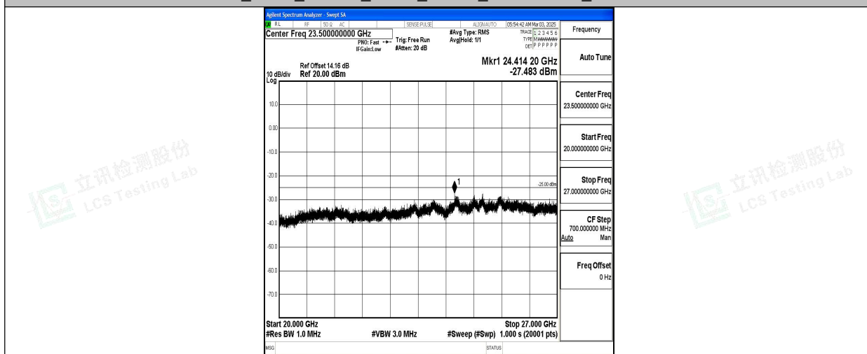
Band7_5MHz_16QAM_21425_1RB#0_20000~27000_20000~27000
