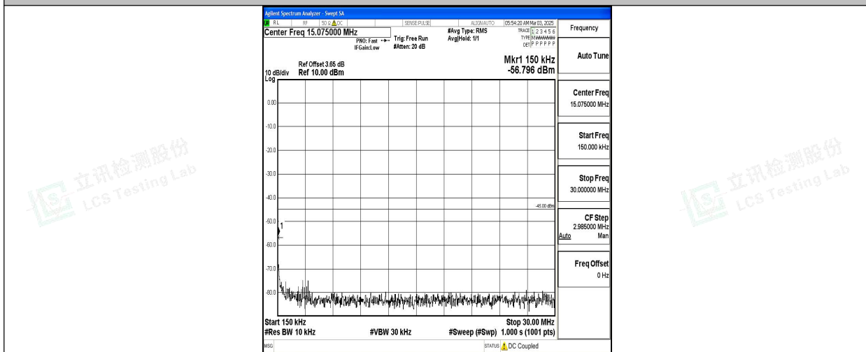
Band7_5MHz_16QAM_21425_1RB#0_0.15~30_0.15~30
