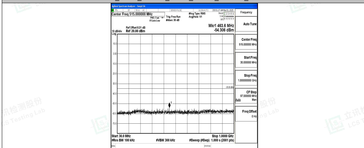
Band7_5MHz_16QAM_20775_1RB#0_30~1000_30~1000
