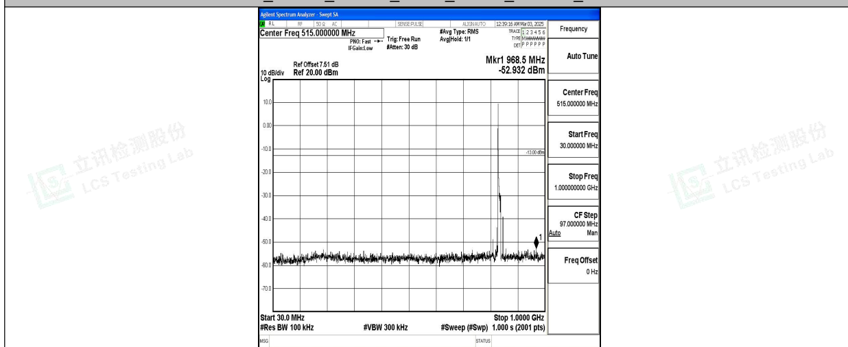
Band5_10MHz_16QAM_20525_1RB#0_30~1000_30~1000
