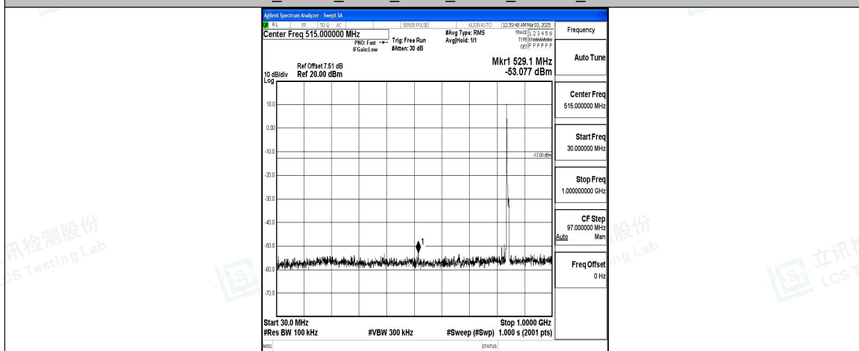
Band5_10MHz_QPSK_20600_1RB#0_30~1000_30~1000
