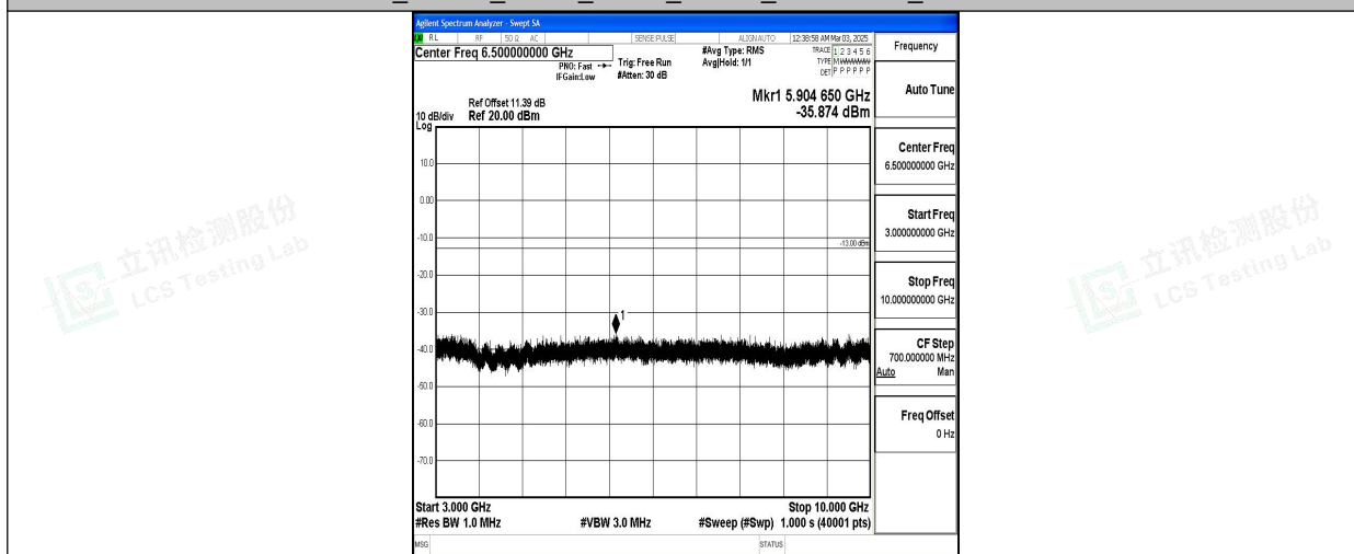
Band5_10MHz_QPSK_20525_1RB#0_3000~10000_3000~10000
