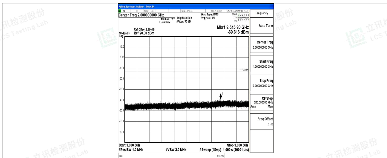
Band5_10MHz_16QAM_20525_1RB#0_1000~3000_1000~3000
