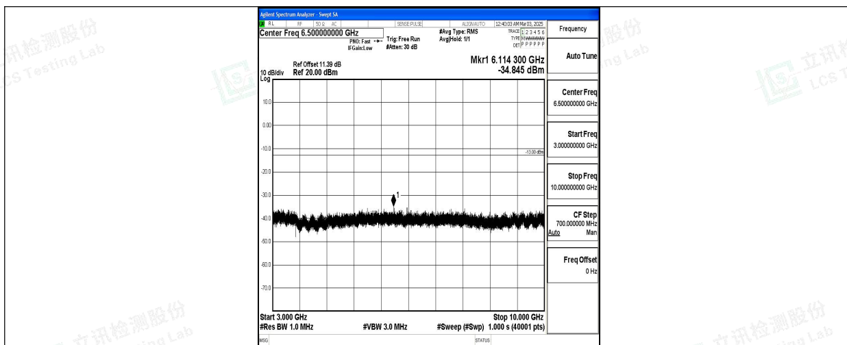
Band5_10MHz_QPSK_20600_1RB#0_3000~10000_3000~10000
