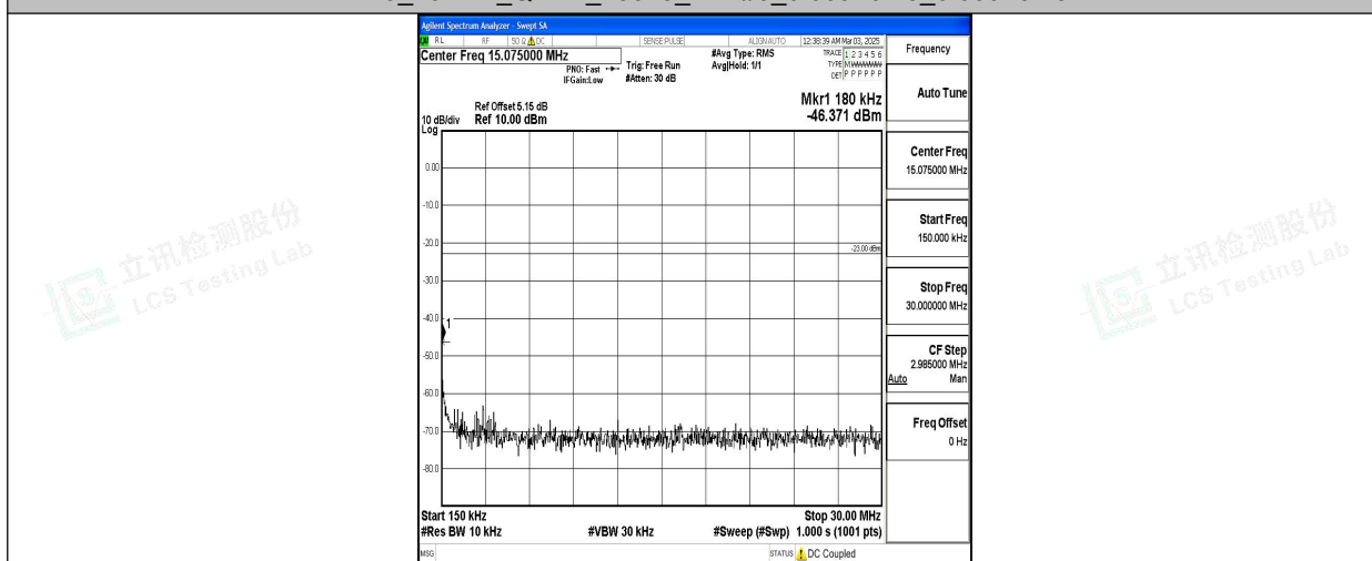
Band5_10MHz_QPSK_20525_1RB#0_0.15~30_0.15~30
