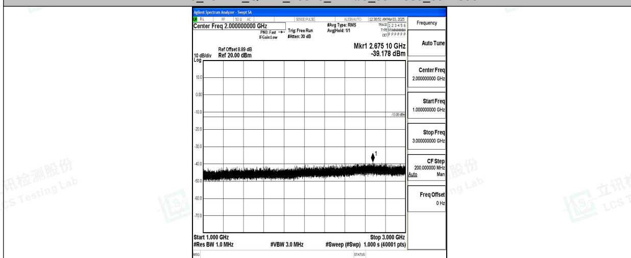
Band5_10MHz_QPSK_20525_1RB#0_1000~3000_1000~3000
