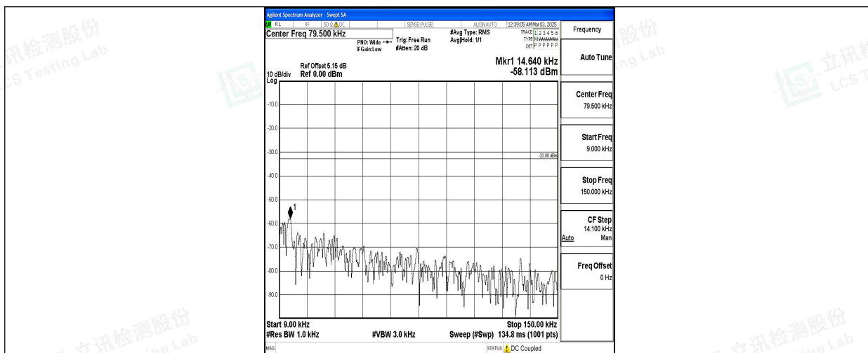
Band5_10MHz_16QAM_20525_1RB#0_0.009~0.15_0.009~0.15
