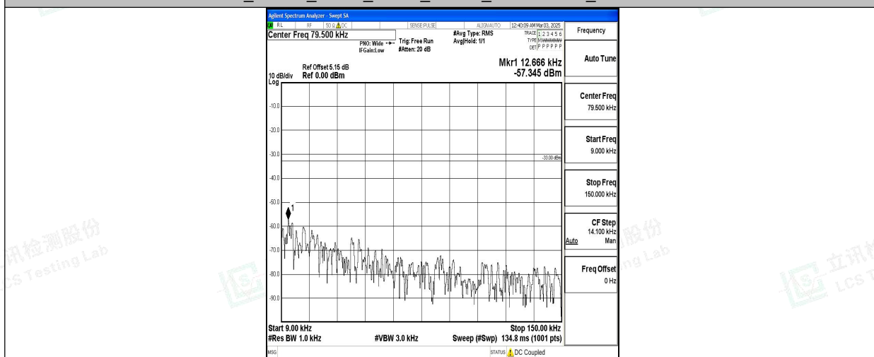
Band5_10MHz_16QAM_20600_1RB#0_0.009~0.15_0.009~0.15
