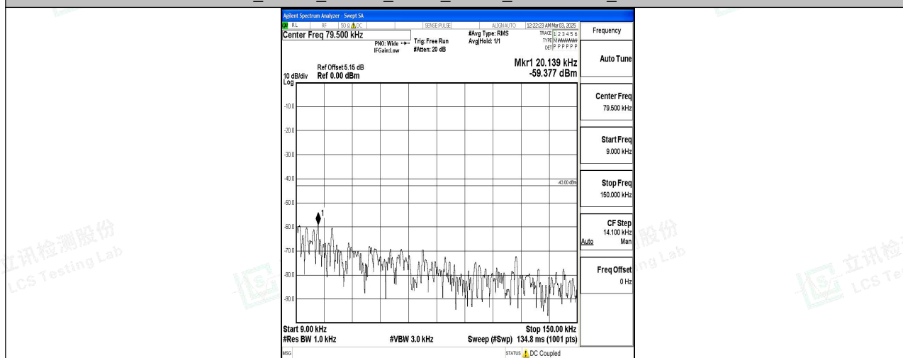
Band4_20MHz_QPSK_20300_1RB#0_0.009~0.15_0.009~0.15
