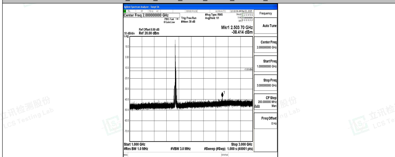
Band4_15MHz_QPSK_20325_1RB#0_1000~3000_1000~3000
