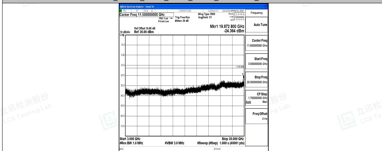
Band4_10MHz_QPSK_20175_1RB#0_3000~20000_3000~20000
