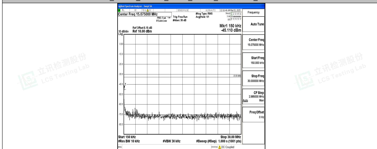
Band4_15MHz_16QAM_20025_1RB#0_0.15~30_0.15~30
