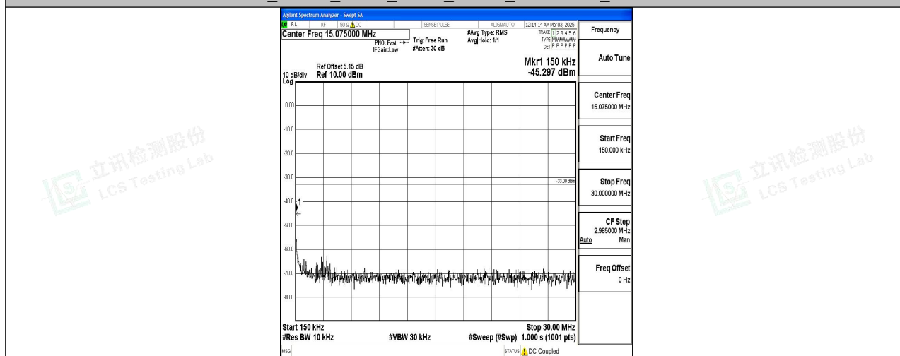
Band4_10MHz_QPSK_20350_1RB#0_0.15~30_0.15~30
