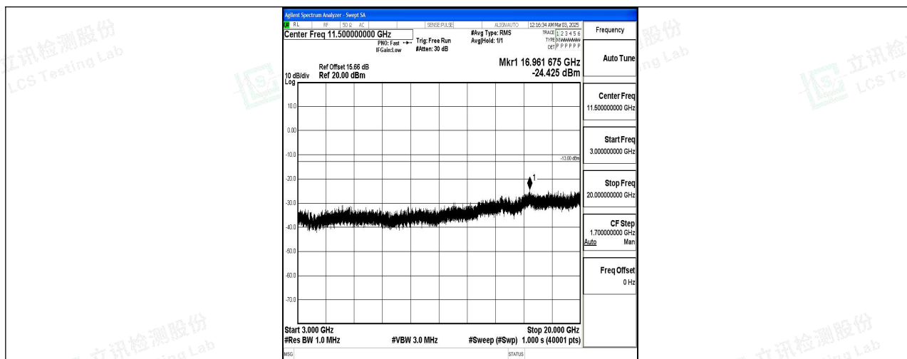
Band4_15MHz_QPSK_20025_1RB#0_3000~20000_3000~20000
