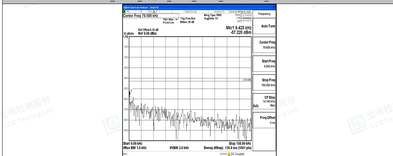
Band4_10MHz_QPSK_20350_1RB#0_0.009~0.15_0.009~0.15
