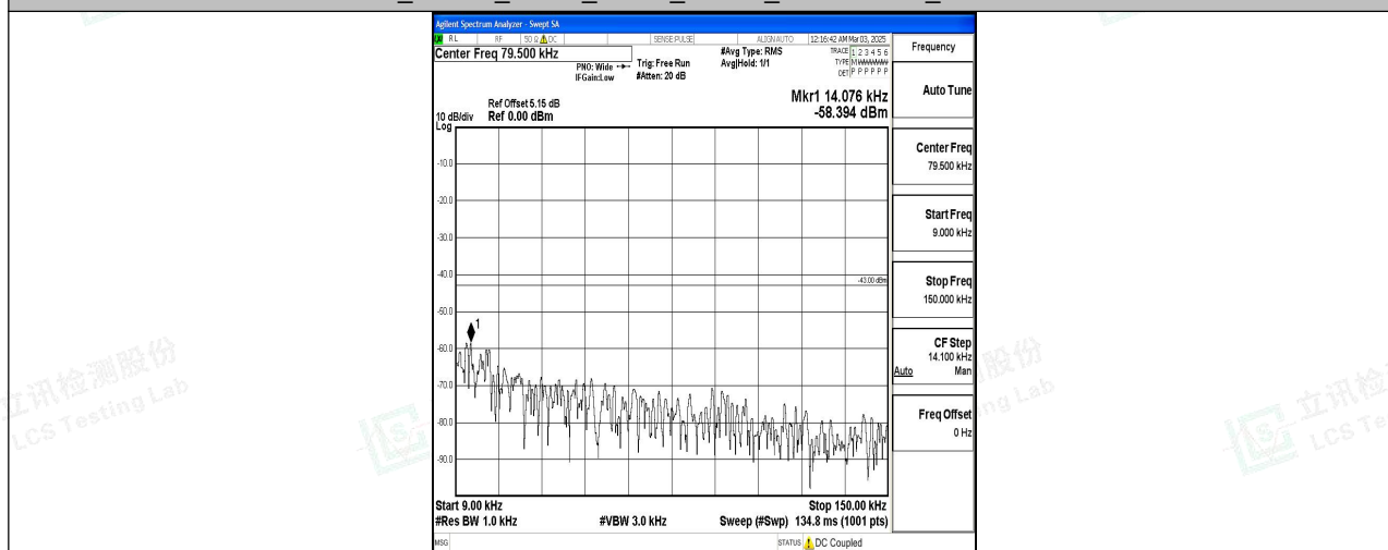
Band4_15MHz_16QAM_20025_1RB#0_0.009~0.15_0.009~0.15
