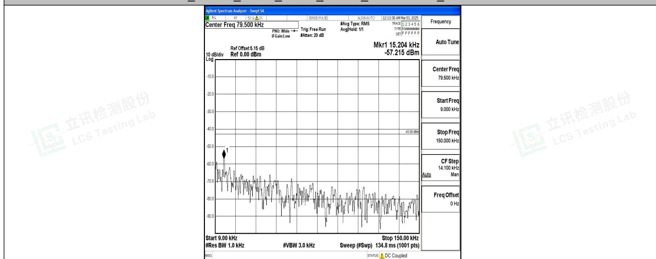
Band4_10MHz_16QAM_20175_1RB#0_0.009~0.15_0.009~0.15
