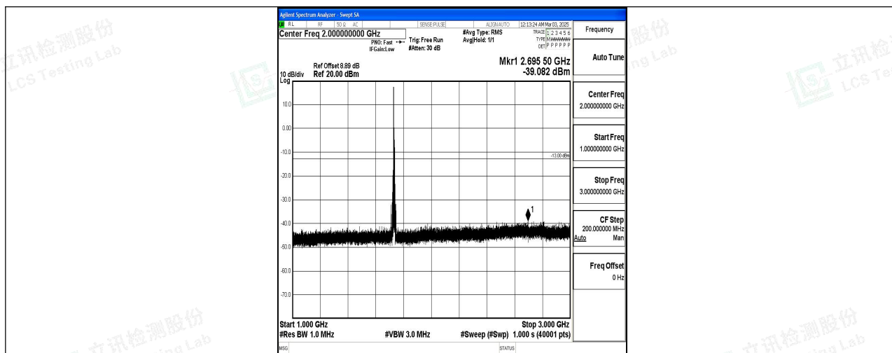
Band4_10MHz_QPSK_20175_1RB#0_1000~3000_1000~3000
