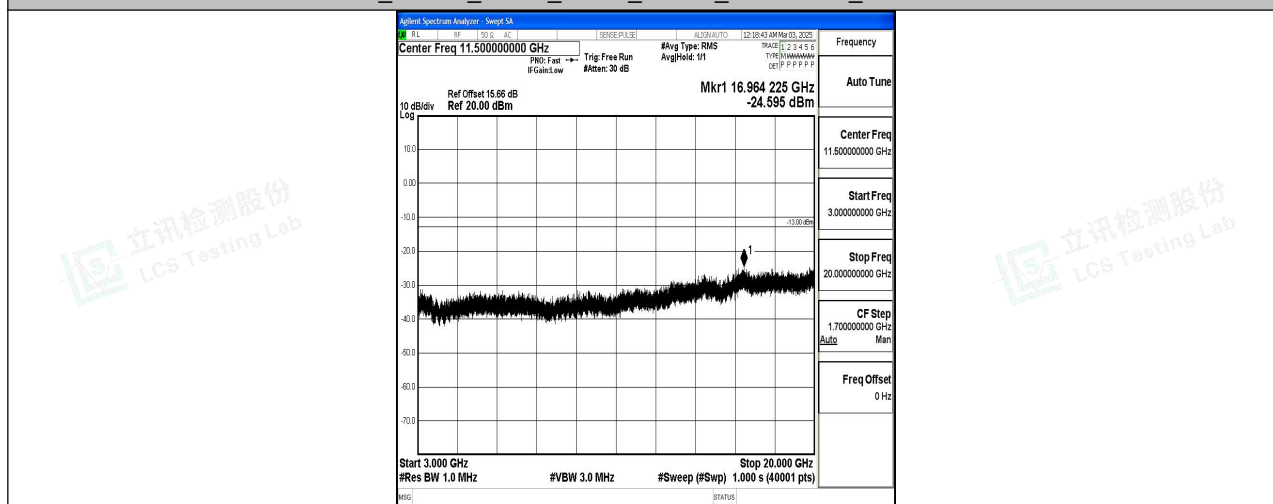
Band4_15MHz_QPSK_20325_1RB#0_3000~20000_3000~20000
