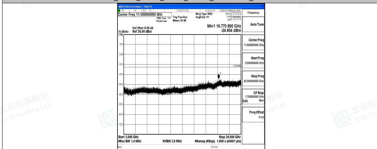
Band4_5MHz_QPSK_20175_1RB#0_3000~20000_3000~20000
