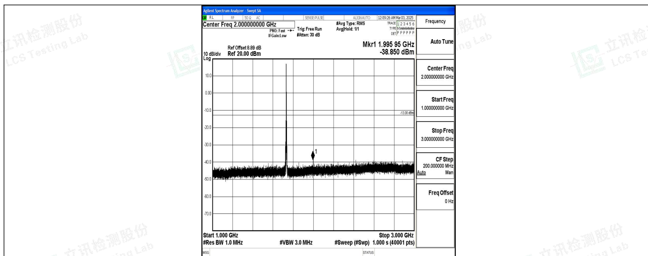
Band4_5MHz_QPSK_20175_1RB#0_1000~3000_1000~3000
