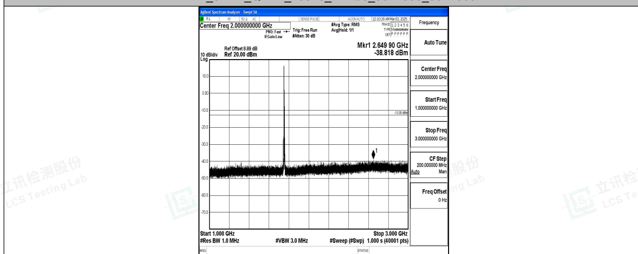
Band4_5MHz_QPSK_20375_1RB#0_1000~3000_1000~3000
