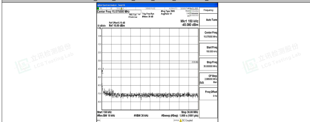
Band4_5MHz_QPSK_20375_1RB#0_0.15~30_0.15~30
