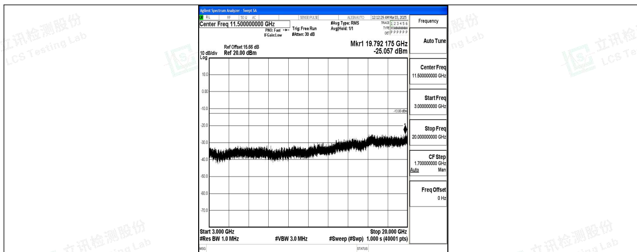
Band4_10MHz_QPSK_20000_1RB#0_3000~20000_3000~20000
