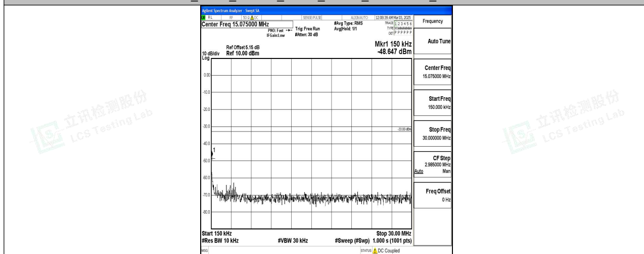
Band4_5MHz_16QAM_19975_1RB#0_0.15~30_0.15~30
