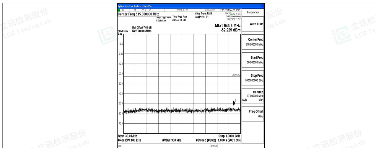
Band4_5MHz_QPSK_20375_1RB#0_30~1000_30~1000
