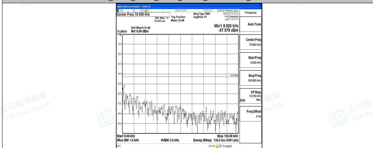
Band4_5MHz_16QAM_19975_1RB#0_0.009~0.15_0.009~0.15
