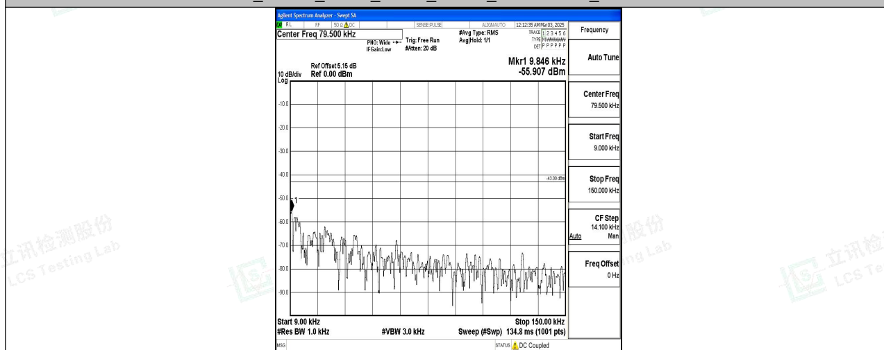
Band4_10MHz_16QAM_20000_1RB#0_0.009~0.15_0.009~0.15
