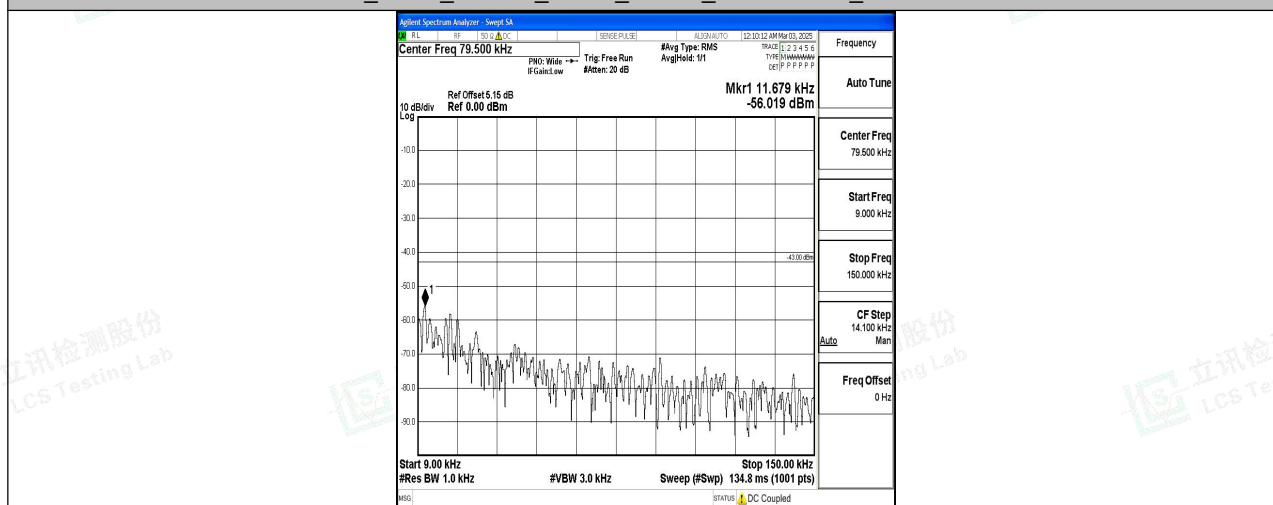
Band4_5MHz_QPSK_20375_1RB#0_0.009~0.15_0.009~0.15
