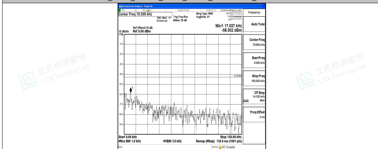
Band4_5MHz_QPSK_19975_1RB#0_0.009~0.15_0.009~0.15
