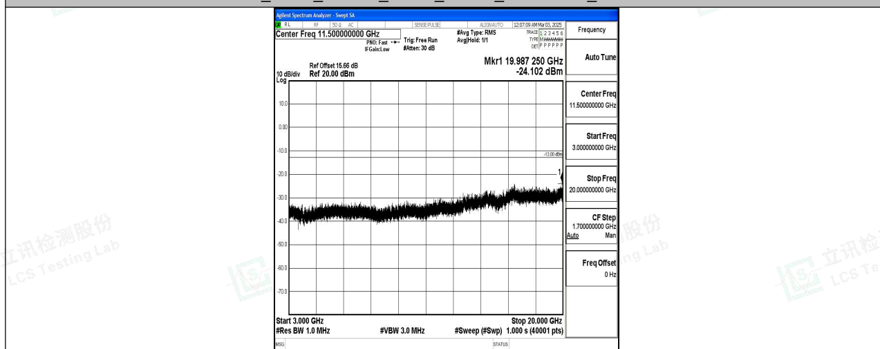
Band4_3MHz_16QAM_20385_1RB#0_3000~20000_3000~20000
