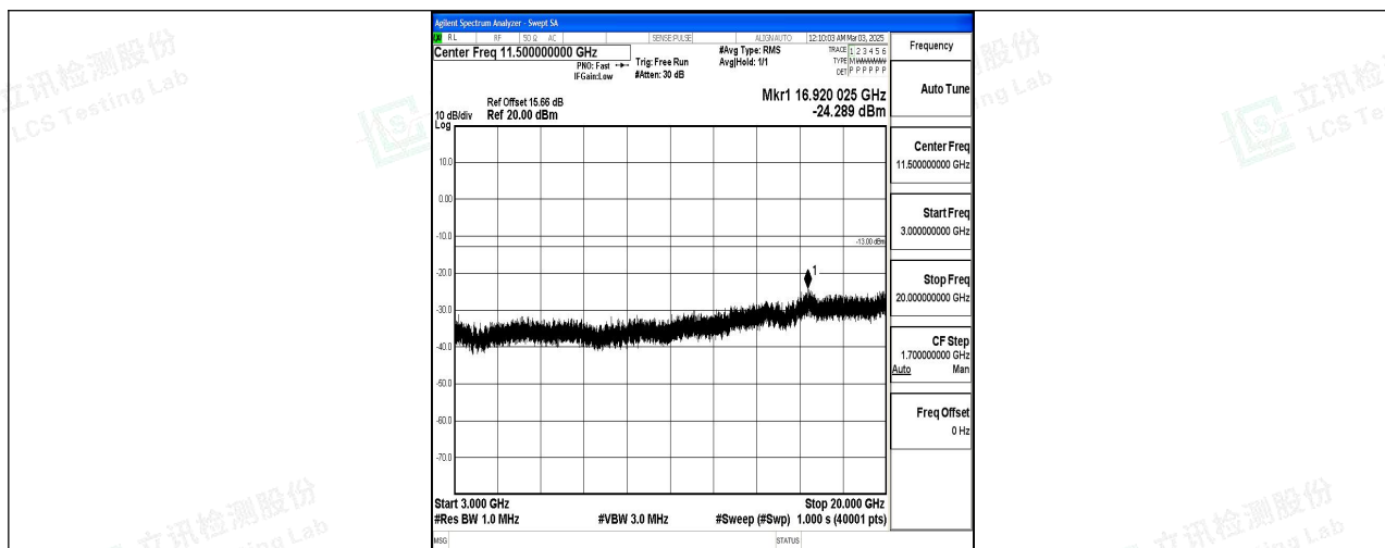
Band4_5MHz_16QAM_20175_1RB#0_3000~20000_3000~20000
