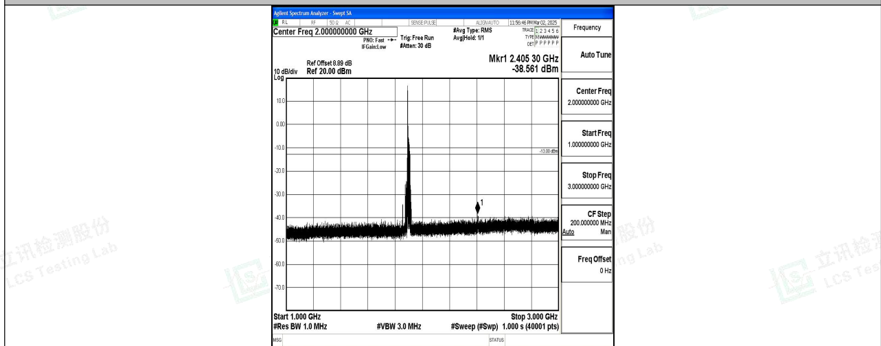
Band2_20MHz_QPSK_19100_1RB#0_1000~3000_1000~3000
