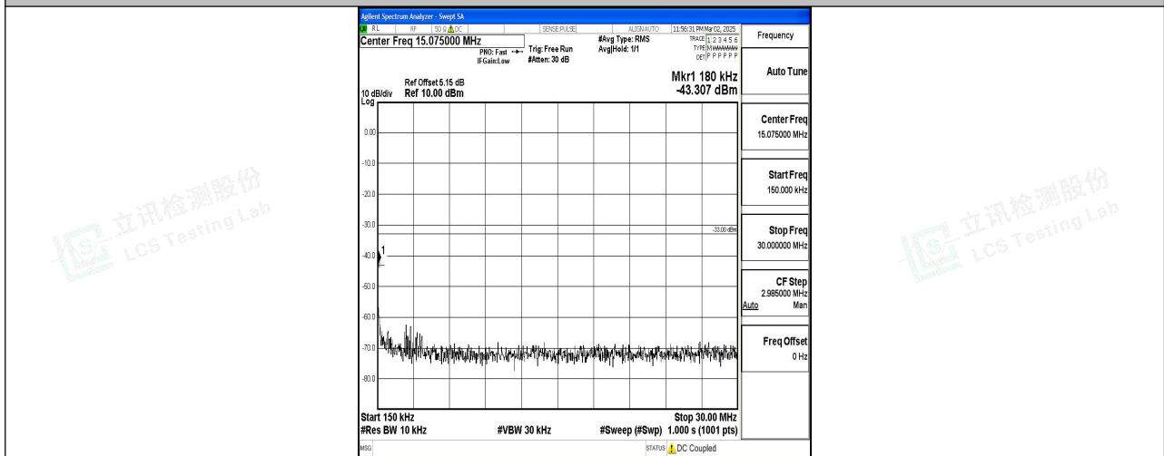
Band2_20MHz_QPSK_19100_1RB#0_0.15~30_0.15~30
