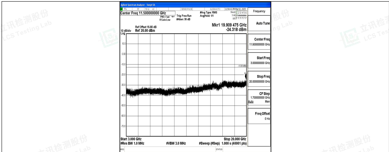
Band2_20MHz_QPSK_18700_1RB#0_3000~20000_3000~20000
