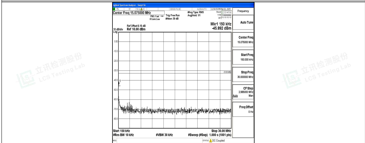
Band2_20MHz_16QAM_18700_1RB#0_0.15~30_0.15~30
