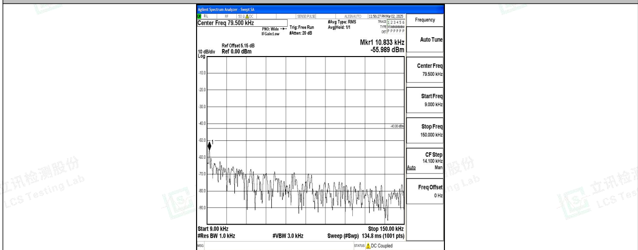
Band2_20MHz_QPSK_19100_1RB#0_0.009~0.15_0.009~0.15
