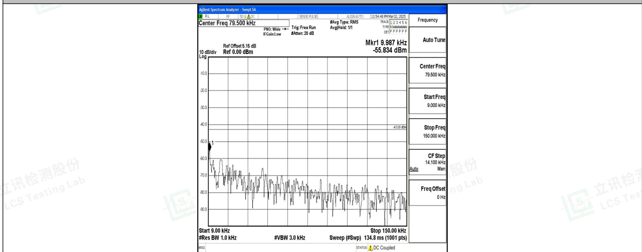
Band2_20MHz_16QAM_18700_1RB#0_0.009~0.15_0.009~0.15
