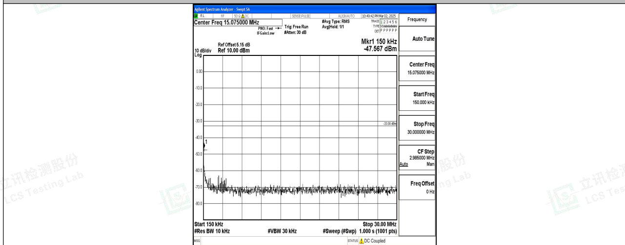
Band2_10MHz_16QAM_19150_1RB#0_0.15~30_0.15~30
