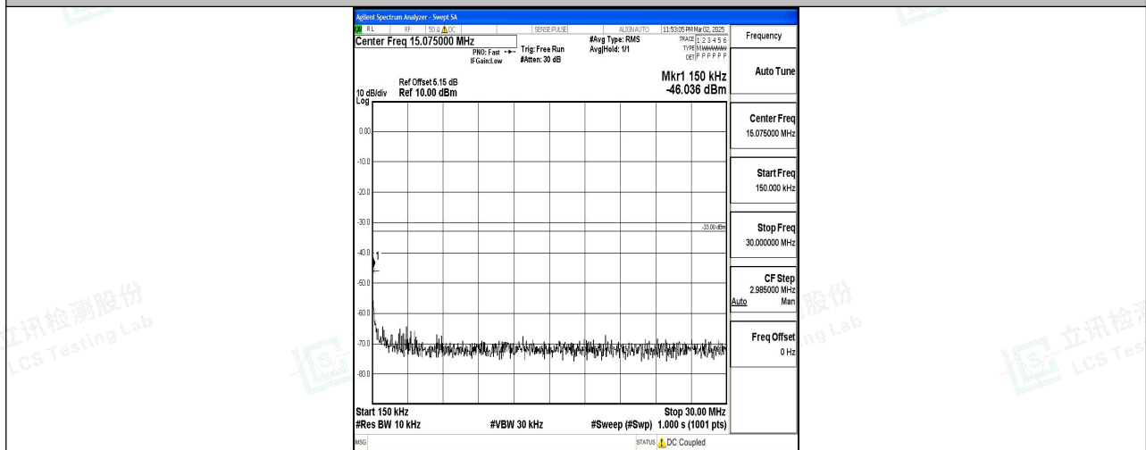
Band2_15MHz_16QAM_19125_1RB#0_0.15~30_0.15~30
