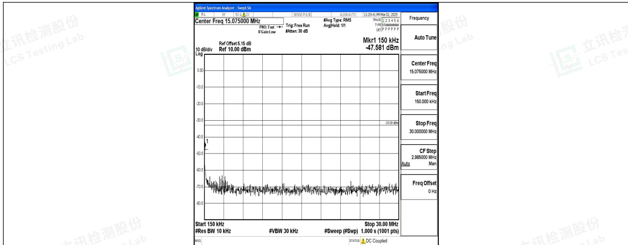
Band2_15MHz_QPSK_18675_1RB#0_0.15~30_0.15~30
