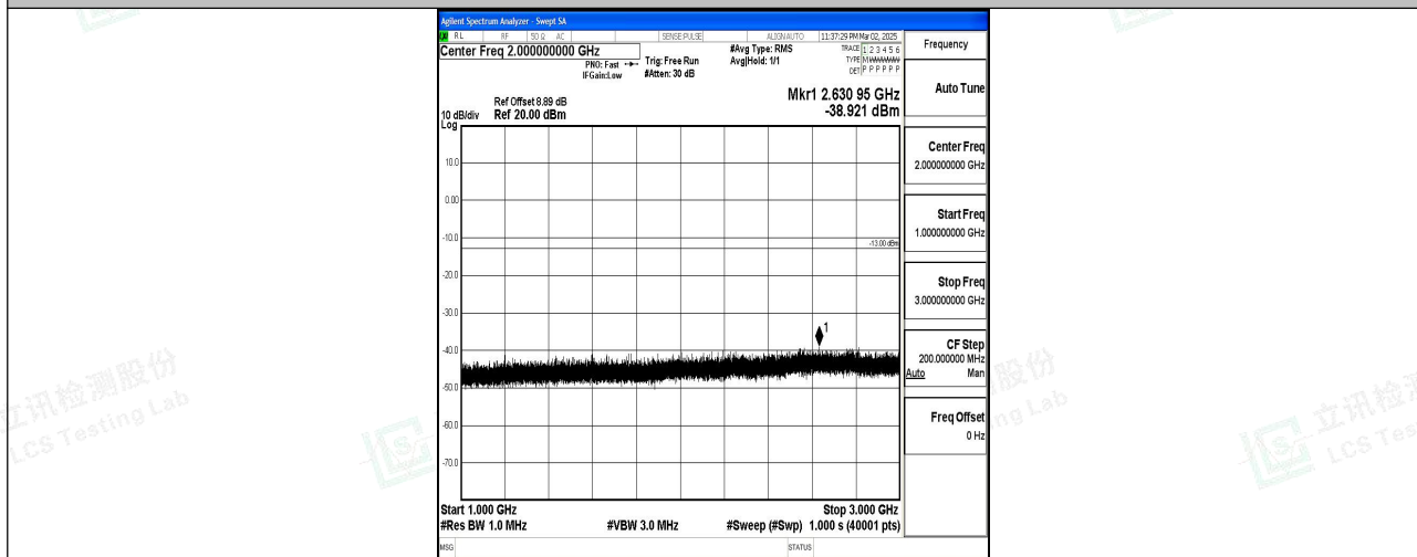
Band2_15MHz_16QAM_18675_1RB#0_1000~3000_1000~3000
