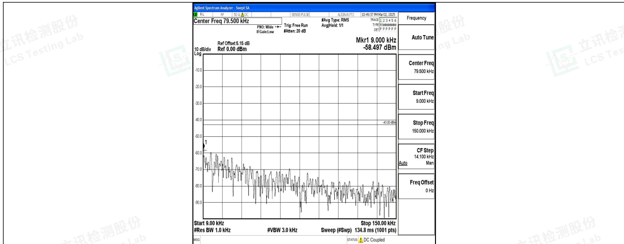
Band2_10MHz_16QAM_19150_1RB#0_0.009~0.15_0.009~0.15
