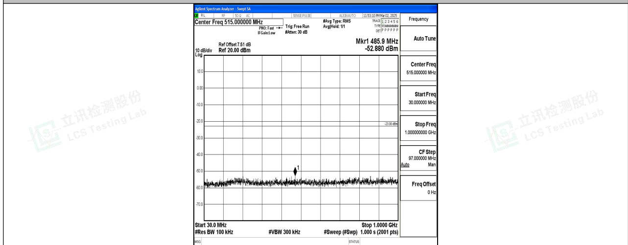
Band2_15MHz_16QAM_19125_1RB#0_30~1000_30~1000
