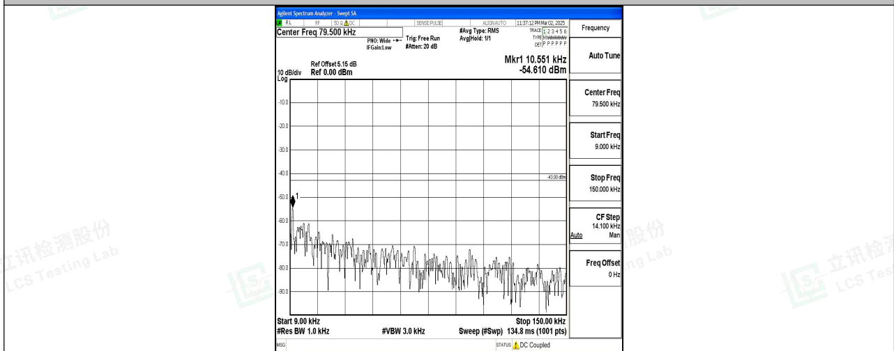
Band2_15MHz_16QAM_18675_1RB#0_0.009~0.15_0.009~0.15
