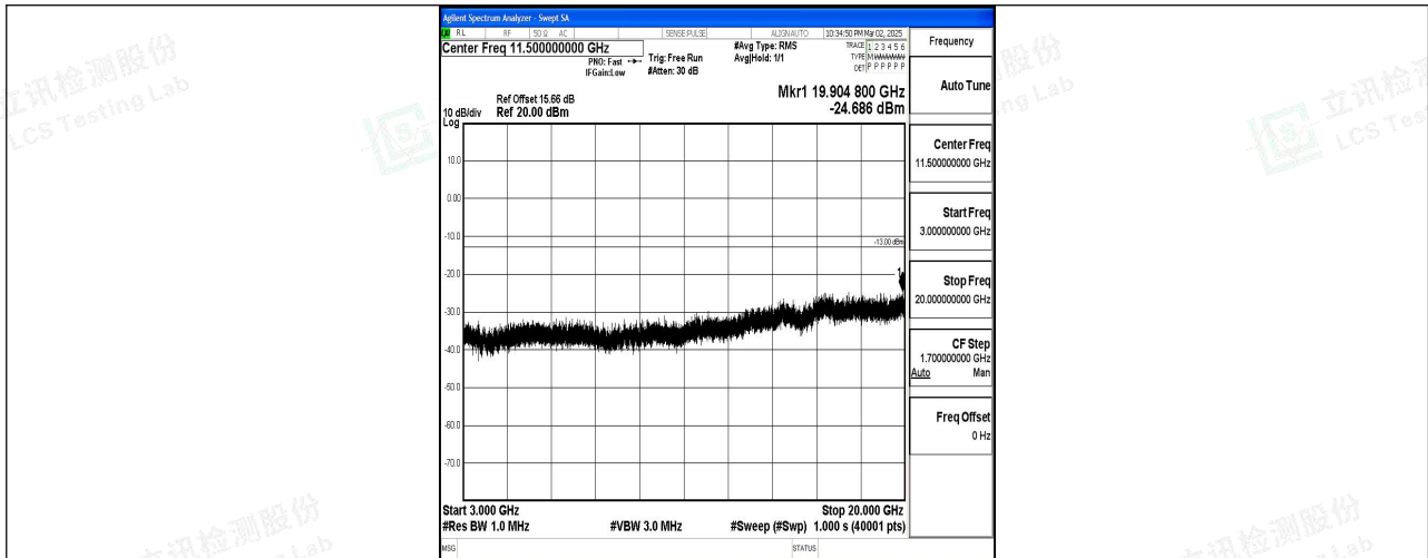
Band2_10MHz_16QAM_18900_1RB#0_3000~20000_3000~20000
