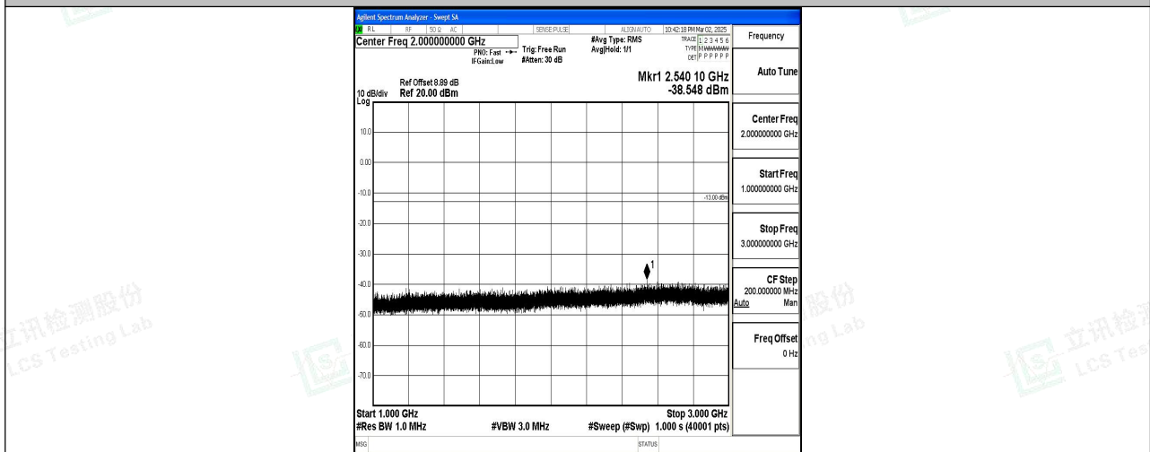
Band2_10MHz_QPSK_19150_1RB#0_1000~3000_1000~3000
