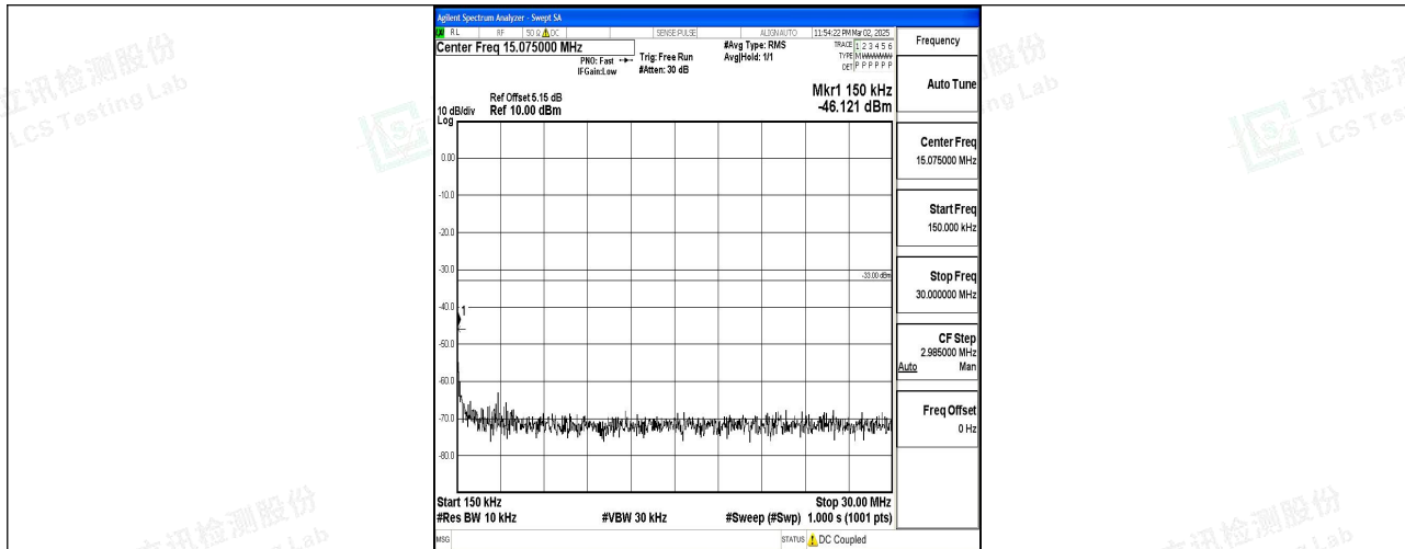
Band2_20MHz_QPSK_18700_1RB#0_0.15~30_0.15~30
