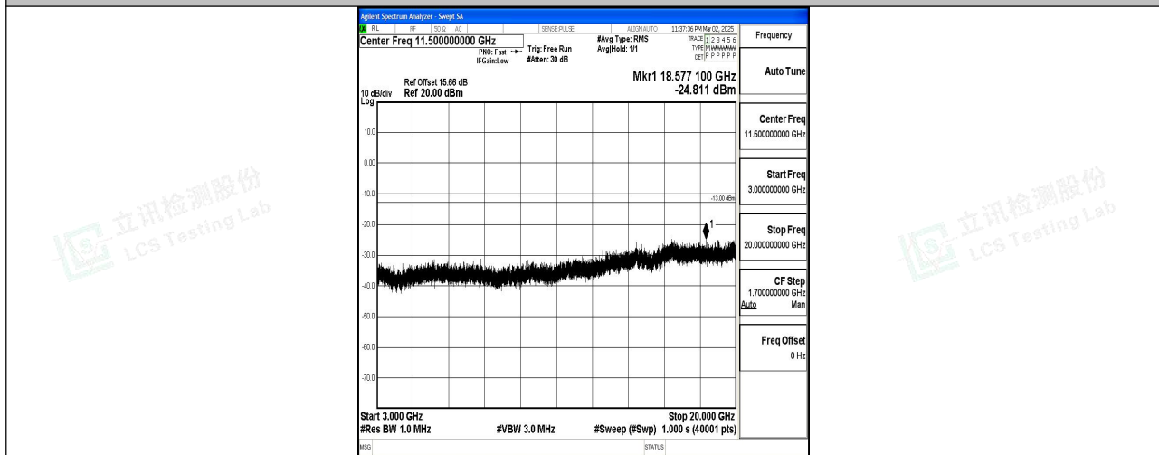
Band2_15MHz_16QAM_18675_1RB#0_3000~20000_3000~20000
