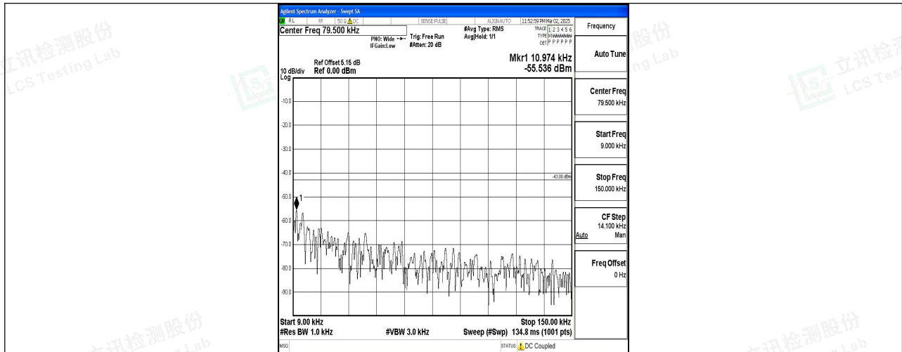
Band2_15MHz_16QAM_19125_1RB#0_0.009~0.15_0.009~0.15
