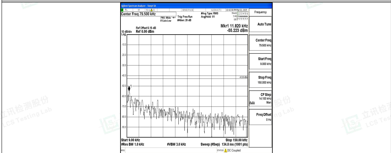
Band2_10MHz_QPSK_19150_1RB#0_0.009~0.15_0.009~0.15
