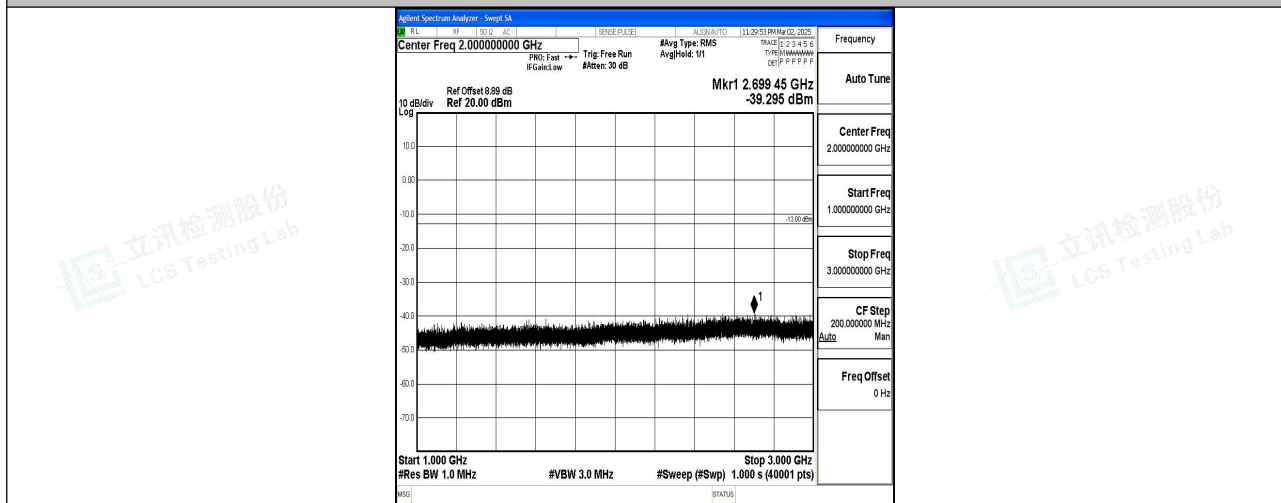
Band2_15MHz_QPSK_18675_1RB#0_1000~3000_1000~3000
