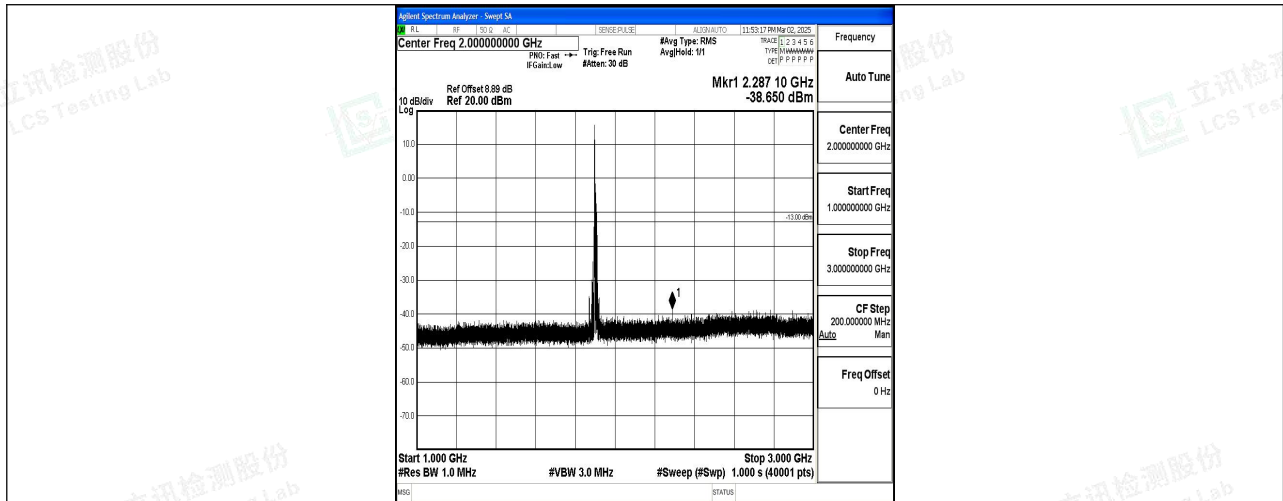
Band2_15MHz_16QAM_19125_1RB#0_1000~3000_1000~3000
