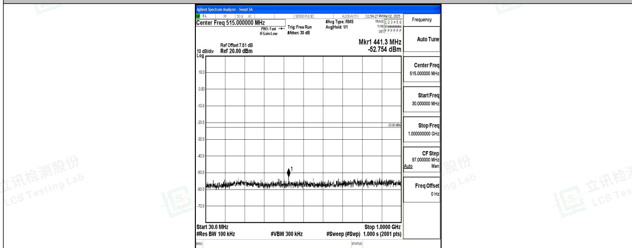
Band2_20MHz_QPSK_18700_1RB#0_30~1000_30~1000
