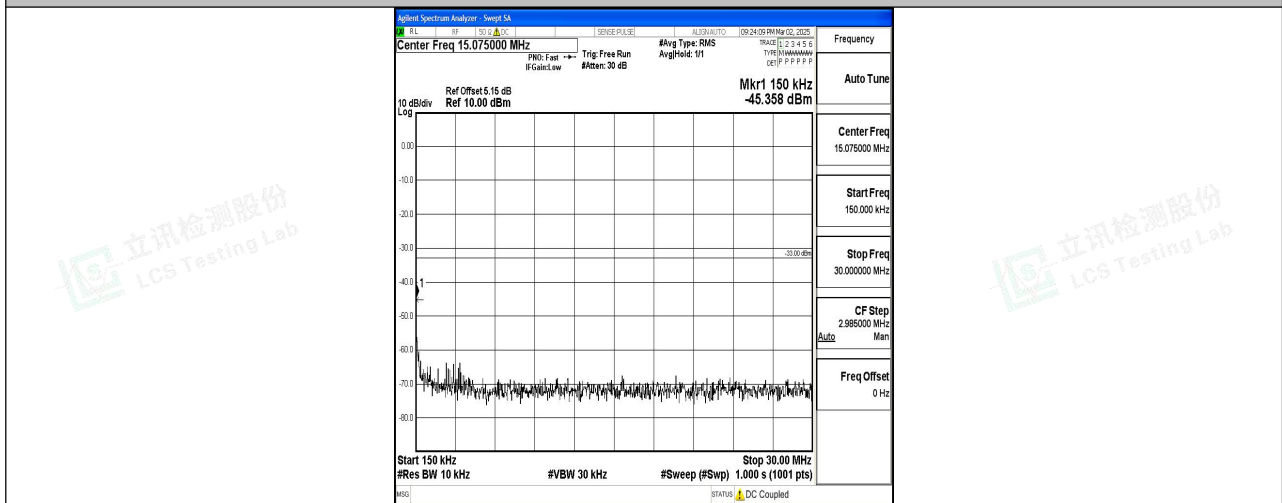
Band2_5MHz_QPSK_19175_1RB#0_0.15~30_0.15~30
