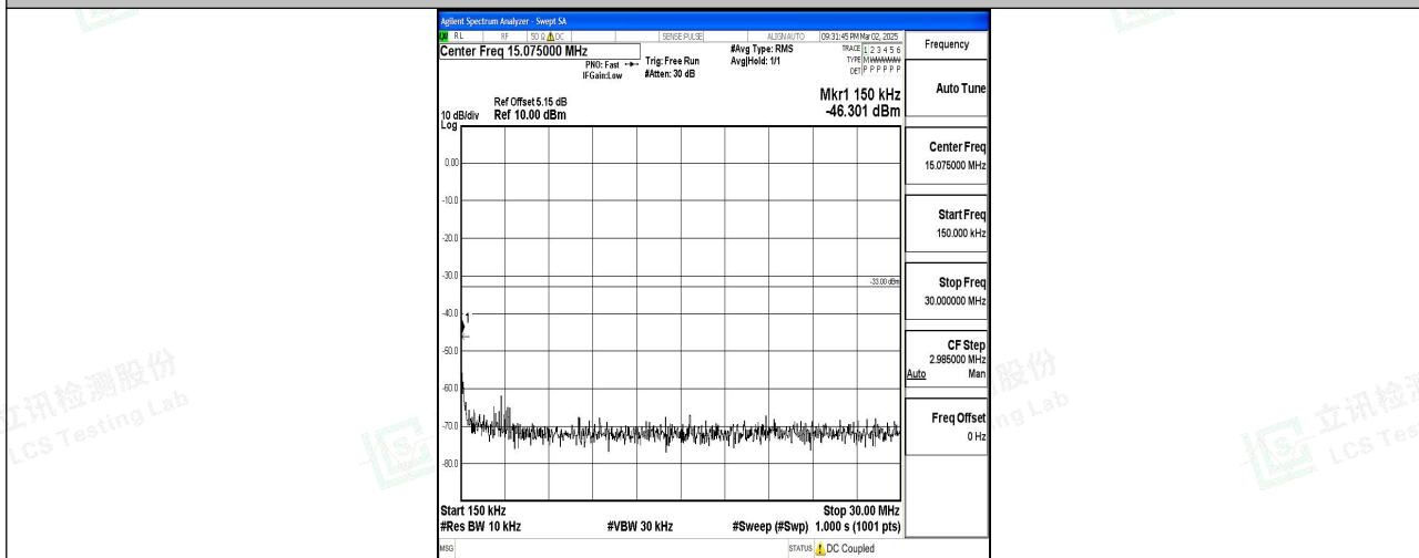
Band2_5MHz_16QAM_19175_1RB#0_0.15~30_0.15~30
