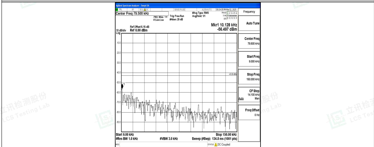
Band2_5MHz_QPSK_19175_1RB#0_0.009~0.15_0.009~0.15
