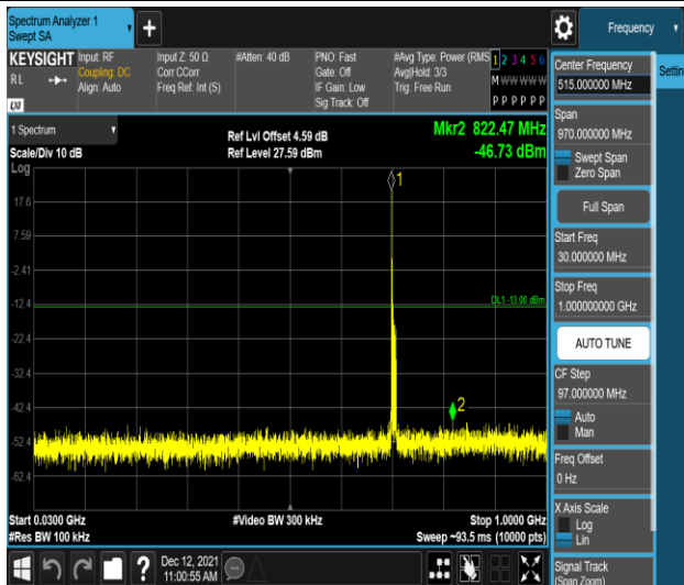
Band17-10MHz-QPSK-23800-1RB#0-Range1:30~1 000MHz
