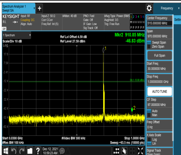
Band17-10MHz-16QAM-23780-1RB#0-Range1:30~ 1000MHz
