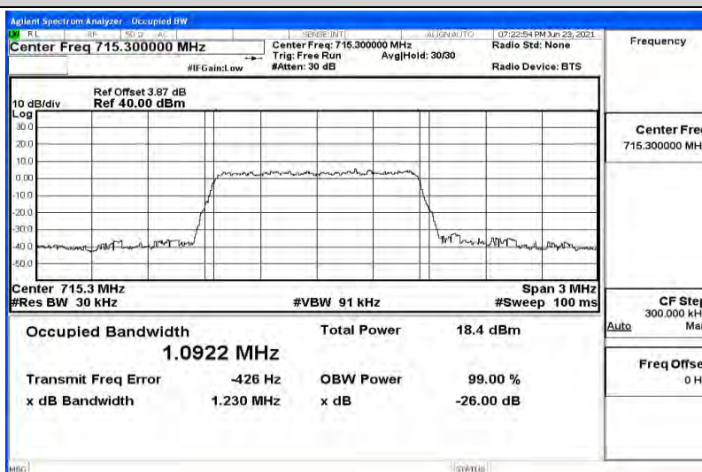
Band12-1.4MHz-QPSK-23173-6RB#0-1.0922
